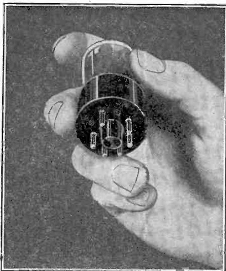
FIG. 8. This is what you see when you remove a 6X5 tube from a receiver and look at its base.
