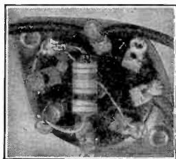
FIG. 16. Actual-size view of a carbon resistor under the chassis.
