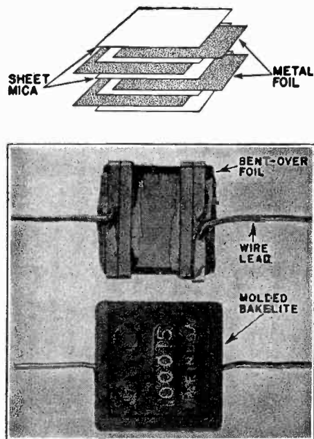
FIG. 20. How a mica condenser is made.
