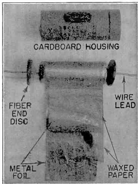
FIG. 19. This photo shows you what's inside a paper condenser. Two long strips of metal foil separated by strips of waxed paper are rolled together, with the two foil strips projecting from opposite ends of the roll and making contact with the two wire leads. The cardboard housing and fiber end discs keep out moisture.
