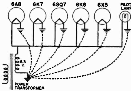
FIG. 24. Filament circuit, with dotted lines indicating the connections which are completed through the chassis of the receiver. All tube filaments and the pilot lamp require 6.3 volts, and the transformer secondary provides this voltage.
