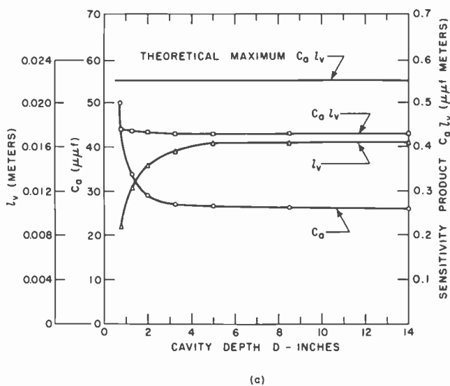
Fig. 5—Low-frequency design parameters, l_v and C_A for (a) flush antenna, and (b) low-silhouette protruding antenna.
