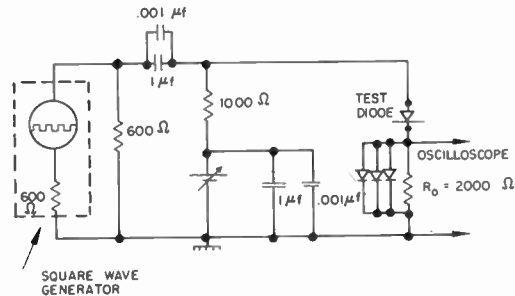
Fig. 6—IBM recovery circuit with semiconductor by-pass diodes.
