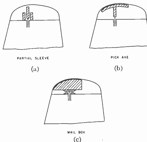
Fig. 24—Typical forms of tail-cap vhf antennas: (a) The partial sleeve antenna, (b) the pickaxe antenna and (c) the mailbox antenna.
