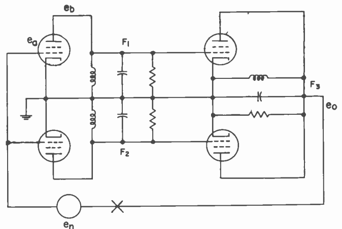
Fig. 2—A parallel-network oscillator employing resonant circuits.
