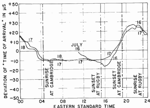
Fig. 5—The diurnal variation of the GBR transmission time, reduced from Fig. 4. The difference in behavior on July 16 and 17, in the interval between 11 h and 18 h EST, is probably caused by an oscillator anomaly.
