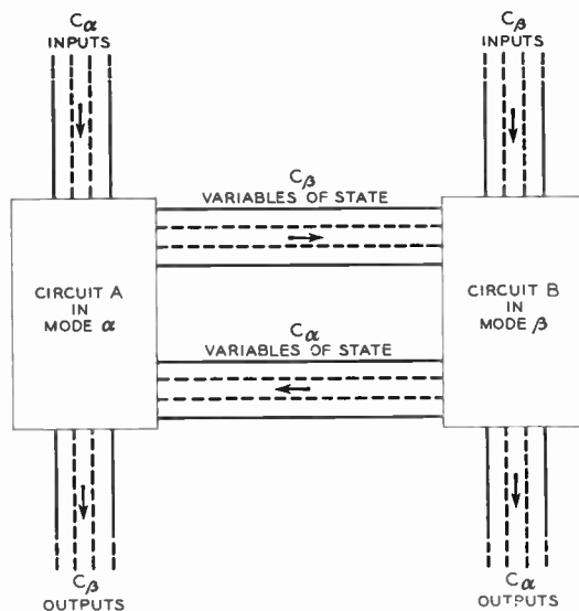
Fig. 16—Block diagram of a two-phase sequential circuit.
