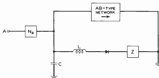
Fig. 9—Representation of the general ABS-type output circuit.
