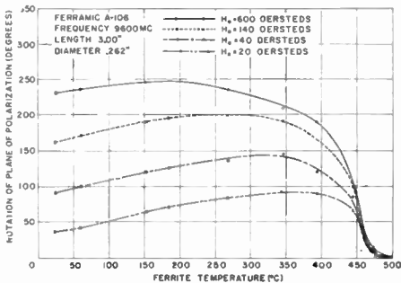
Fig. 1—Temperature dependence of the rotation of plane of polarization in Ferramic A-106, with applied magnetic field as parameter.
