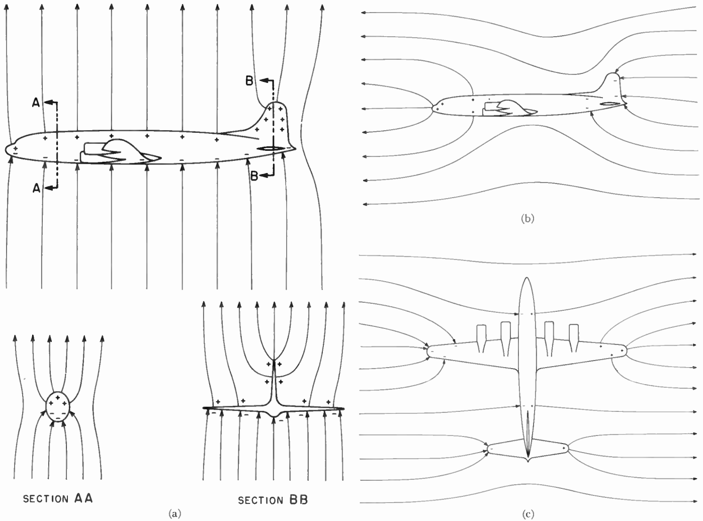
Fig. 2—Field fringing and airframe charging produced by incident electric fields in (a) the vertical direction, (b) the longitudinal direction, and (c) the transverse direction.
