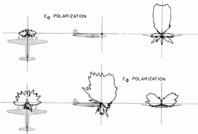
Fig. 25—Radiation patterns of a ram's-horn VOR antenna located on top centerline near nose of a DC-6B aircraft. Horizontal-plane E_{\phi} polarization pattern shows response to signals of interest.
