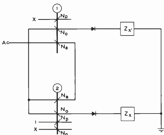
Fig. 8—A two-position AB-type switch.
