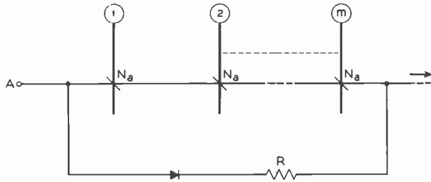
Fig. 20—Resistive shunt for adjustment of the switching time.
