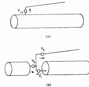
Fig. 10—Illustrating the decomposition of an idealized fixed-wire, airframe combination into transmission line and antenna modes.
