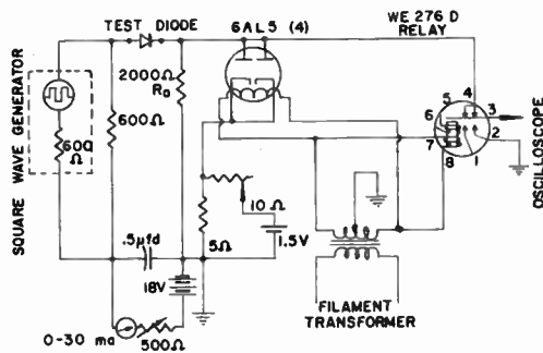
Fig. 8—Modified IBM circuit.
