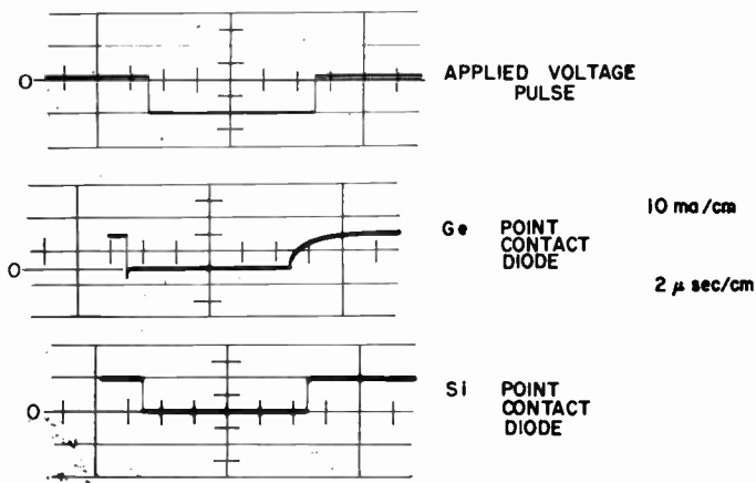
Fig. 2—Pulse response.
