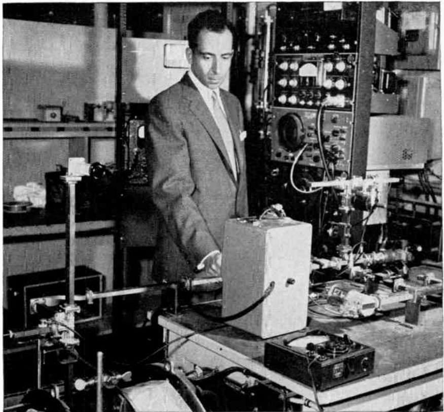
Studying ferromagnetic resonance. A cavity perturbation method is used, in which a ferrite specimen placed in a high Q microwave cavity changes cavity properties in accordance with electrical and magnetic properties of the material.
