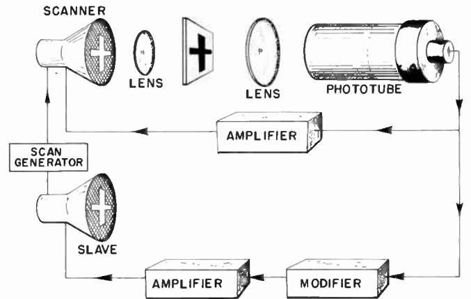
Fig. 3—Block diagram of experimental image processing system. Feedback around the fluorescent screen of the scanning cathode ray tube is accomplished by feeding the amplified phototube signal to the scanner. This signal is also modified and the resulting picture is displayed on the slave cathode-ray tube screen.
