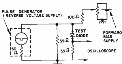
Fig. 1—Circuit for observing pulse response and recovery dependence on forward current.
