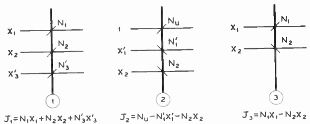
Fig. 5—Schematic and algebraic representations of input leads and windings on magnetic cores.
