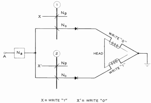
Fig. 11—Circuit for writing on a magnetic drum.
