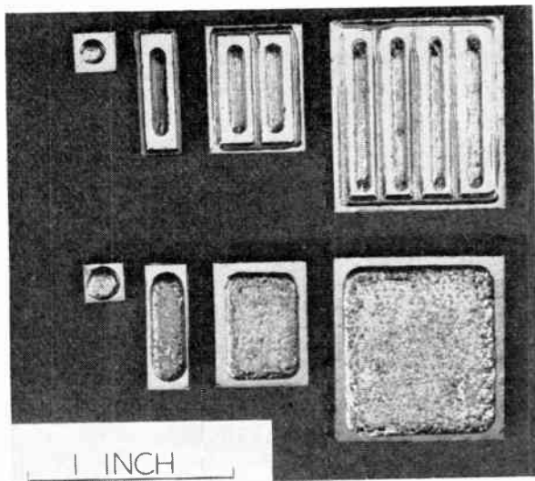
Fig. 6—Transistor types: (left to right)—(1)X-78 standard power transistor (without base electrode); (2) single-bar transistor; (3) double-bar transistor; (4) multi-bar transistor. The upper row shows the emitter-base side of the transistors and the lower row the collector side.
