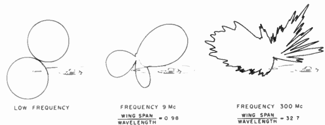
Fig. 1—Typical radiation patterns of a tail-cap antenna on a DC-4 aircraft in (a) the low-frequency range, (b) the longitudinal resonance range, and (c) the transverse resonance or diffraction range.
