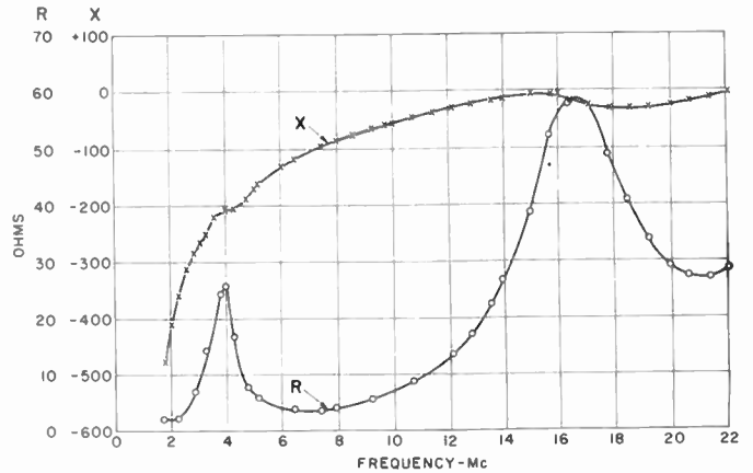
Fig. 12—Input impedance of 7-foot tail-cap antenna on DC-4 aircraft.
