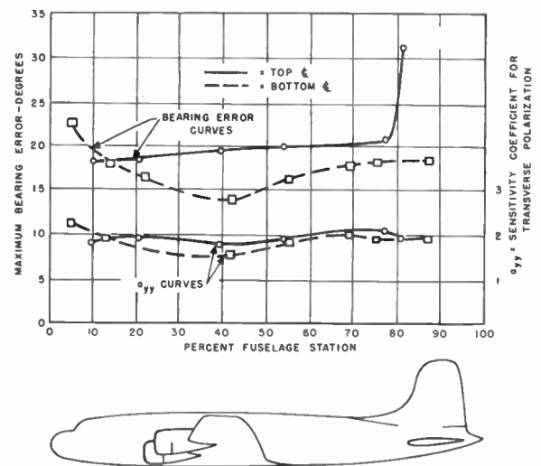
Fig. 7—Low-frequency loop antenna survey data for DC-4 aircraft showing maximum bearing error and sensitivity coefficient for transverse polarization for top and bottom centerline locations.
