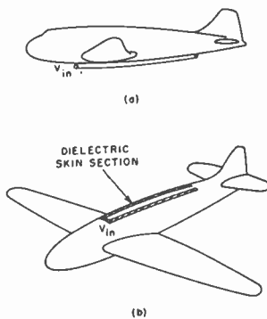
Fig. 14—Increasing the effectiveness of coupling to airframe resonances with fixed-wire type exciters, (a) by use of a large diameter feed wire and (b) by use of a wide flush strap rather than a wire
