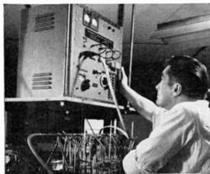
Glennite 1 MC Incremental Capacitance Ratio Bridge
