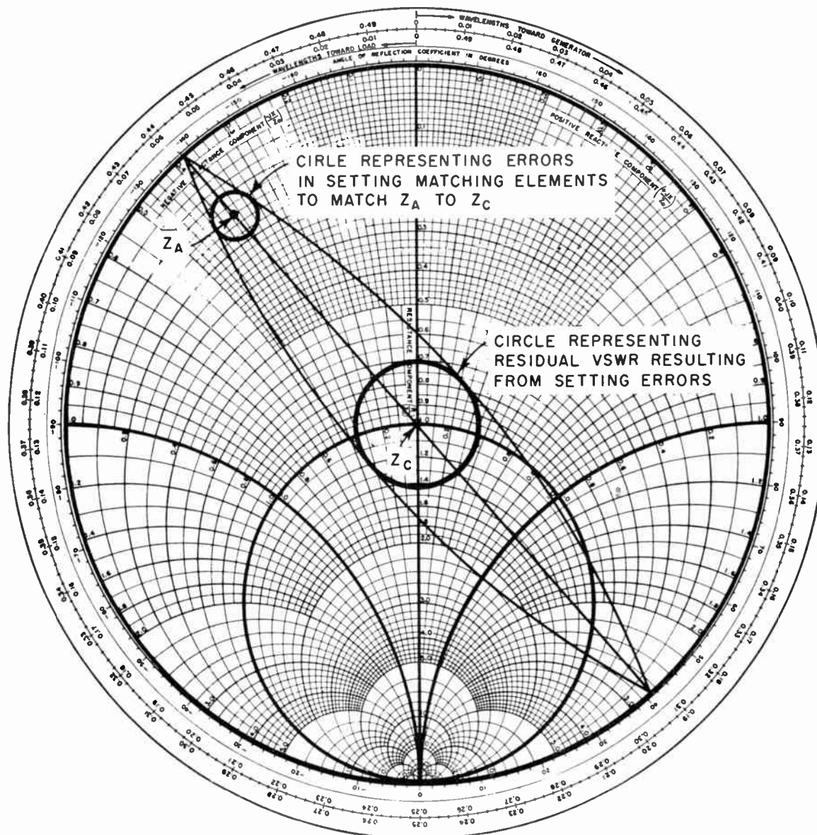
Fig. 19—Smith chart construction relating residual VSWR to error in setting network elements in a dissipationless matching circuit.
