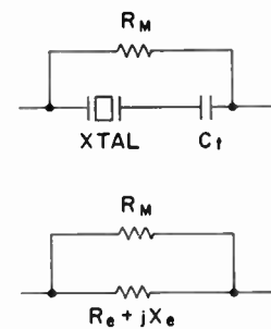
Fig. 8—Crystal unit with mode-suppression resistor.
