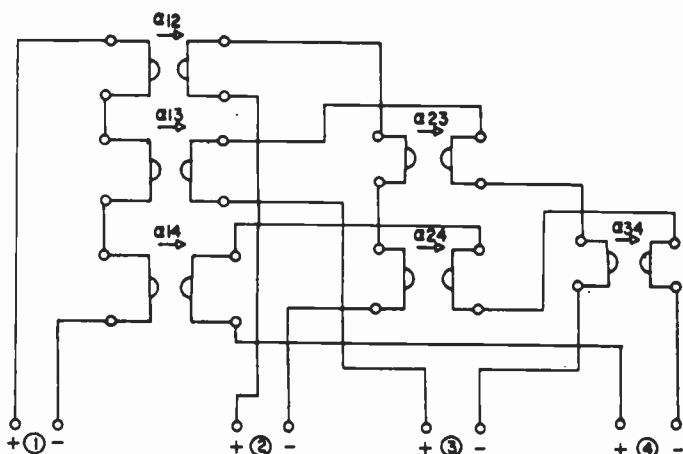
Fig. 2—Four-port all-gyrator network.
