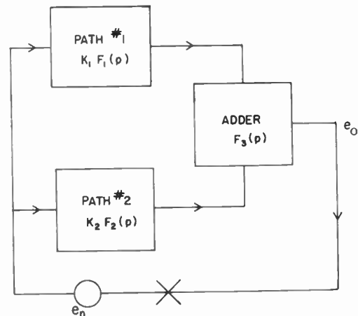
Fig. 1—Block diagram of the general parallel-network oscillator.
