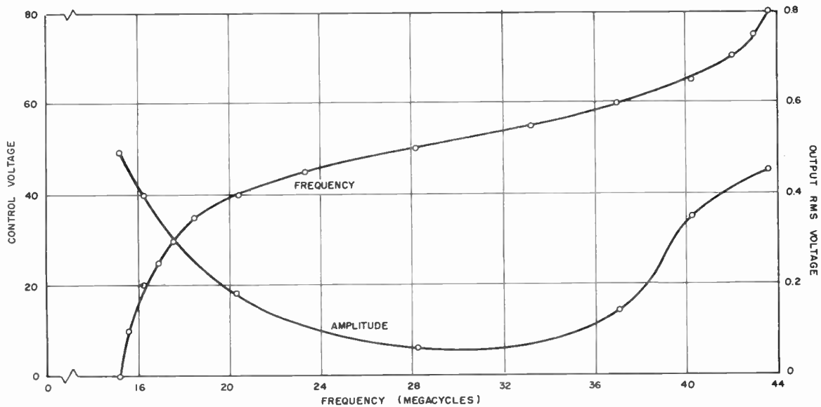
Fig. 9—Tuning characteristics of oscillator employing lead and lag networks.
