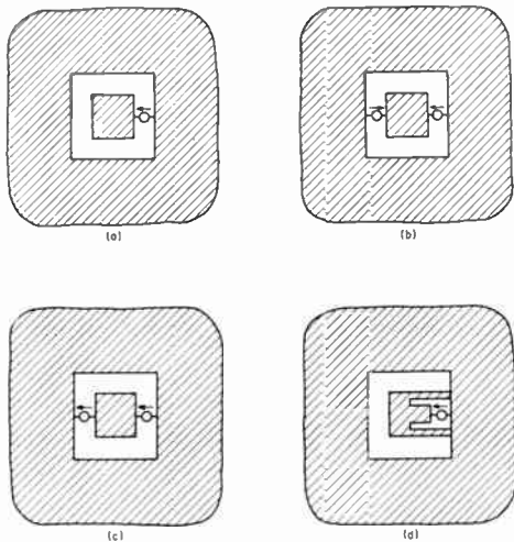
Fig. 28—The modes of operation of a patch antenna and the related E -fed cavity antenna: (a) the patch antenna, (b) anti-symmetric mode, (c) symmetric mode, and (d) the E -fed antenna.
