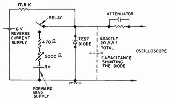
Fig. 10—Bell Telephone Laboratories recovery circuit.
