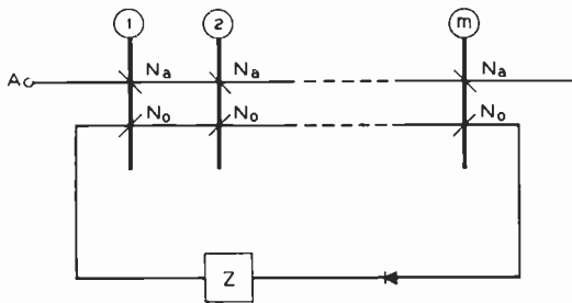
Fig. 6—A simple T-type output circuit with a passive load, Z .
