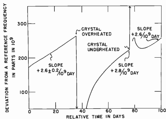
Fig. 1.—Examples of the effects of temperature discontinuities on the frequency of a crystal oscillator.
