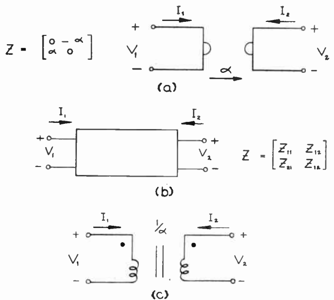
Fig. 1—Reciprocal and non-reciprocal circuits. (a) Gyrator. (b) General two-port. (c) Ideal Transformer.
