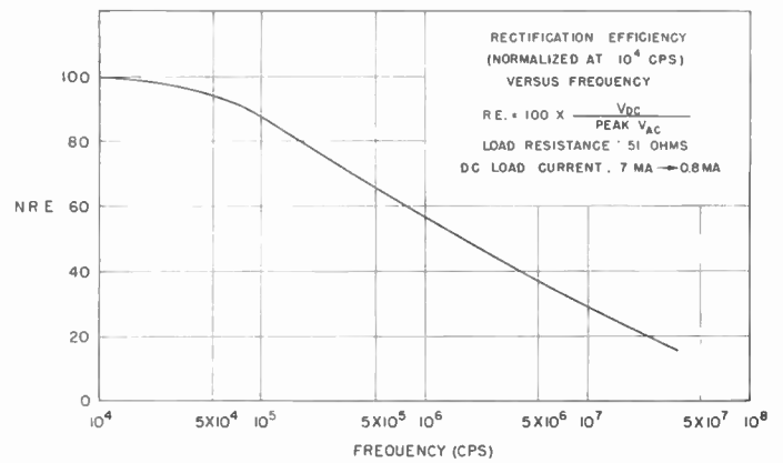
Fig. 12—Rectification efficiency vs frequency for heavily-loaded diode, normalized to 10^4 cps.
