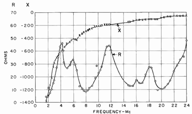
Fig. 13—Input impedance of 2-foot wing-cap antenna on DC-4 aircraft.
