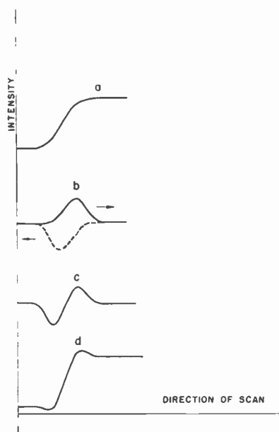
Fig. 7—Practical realization of contour enhancement by one differentiation only. (a) A somewhat degraded picture signal of a transition between two levels. (b) The derivative of this signal, but delayed slightly in the direction of scan. The dotted line refers to the return signal. (c) The algebraic sum of the two signals shown in (b). This is approximately equal to an undelayed negative second derivative signal. (d) The sum of the signal shown in (c) and that shown in (a).
