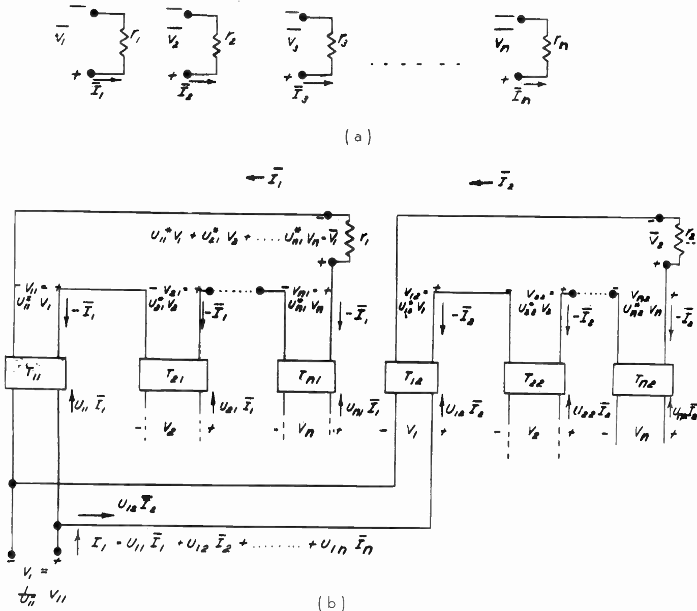
Fig. 3—Synthesis of non-reciprocal network. (a) Resistor network for diagonalized impedance matrix. (b) General circuit for an hermitian impedance matrix.
