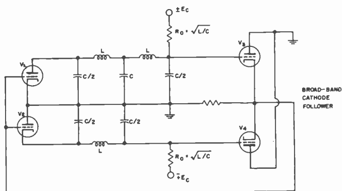
Fig. 4—A parallel-network oscillator employing artificial transmission lines.
