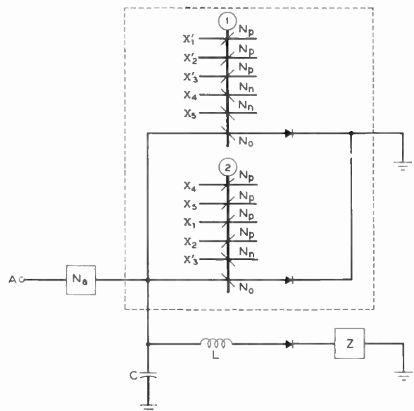
Fig. 12—An ABS-type checking circuit for a two-out-of-five code.
