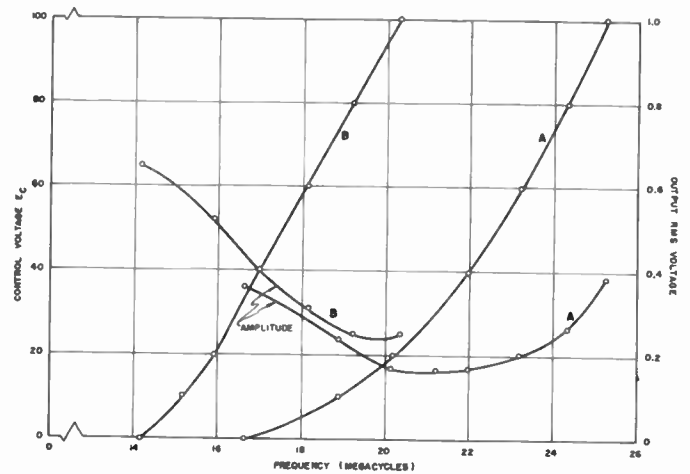
Fig. 7—Tuning characteristics of transmission line type oscillator.
