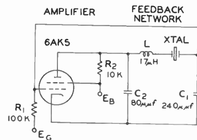
Fig. 1—Simplified schematic of single-tube crystal oscillator.
