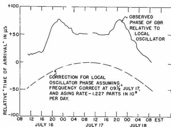
Fig. 4—The relative phase variation of GBR over a period of nearly 48 hours. The lower curve gives the presumed phase variation of the GBR frequency source relative to the local oscillator.
