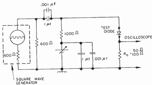
Fig. 4—Circuit for observing the effect of different diode-loop resistances.
