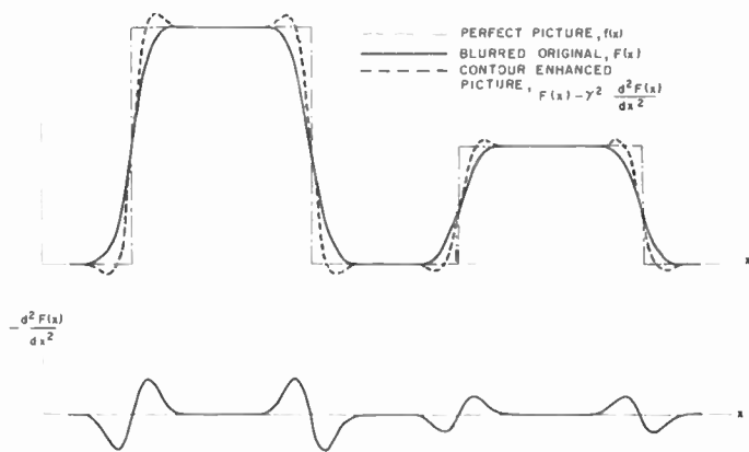
Fig. 5—Principle of contour enhancement. The upper part shows three pictures functions: one is the perfect picture signal, the second is the picture signal from the degraded original, and the third shows a partial restoration towards the perfect picture signal. The lower figure shows the negative second derivative of the original signal that was added as a correction signal to the signal from the degraded original.
