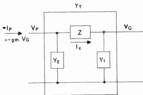
Fig. 7—Equivalent circuit of the oscillator.
