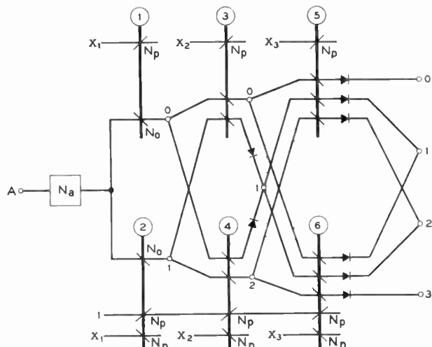
Fig. 15—A three-variable AB-type symmetric switch.
