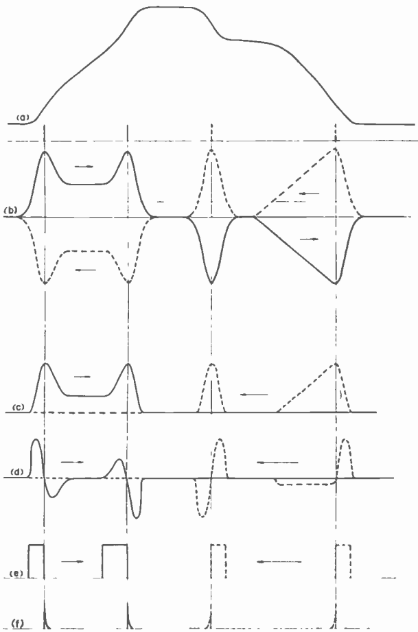
Fig. 9—Practical contour outlining procedure. The procedure consists of obtaining an outline at the points where the slope of the video signal has a local maximum exceeding a threshold value. The steps are indicated below. The forward scan is shown in solid lines and the return traces with dotted lines. (a) Original picture signal, (b) first derivative, (c) rectification with bias, (d) second derivative (when first derivative exceeds threshold), (e) trigger driven by (d), (f) pulses, differentiated and rectified (e).
