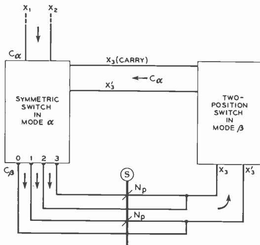
Fig. 18—Block diagram of a two-phase serial binary adder.
