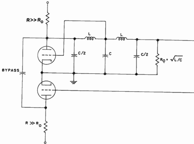
Fig. 5—Simplification of the oscillator employing artificial transmission lines.
