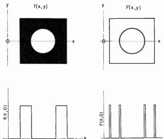
Fig. 8—Principle of contour outlining. The upper part shows a picture and its derived outline. The lower part shows the corresponding video signals across a single scan ( y = 0 ).
