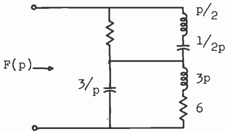
Fig. 1—Realization of F(p) = \frac{p^2 + 3p + 7}{p^2 + 2p + 1} .
