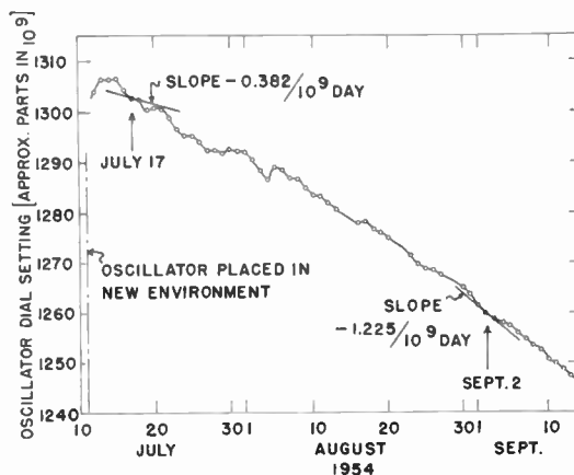
Fig. 8—History of the Cambridge oscillator relative to the MSF daily transmissions at 60 kc. Note that slopes derived from the parabolas of Figs. 4 and 6 are in approximate agreement with the curve for July 17 to 18 and Sept. 1 to 3, but not for July 16 to 17.
