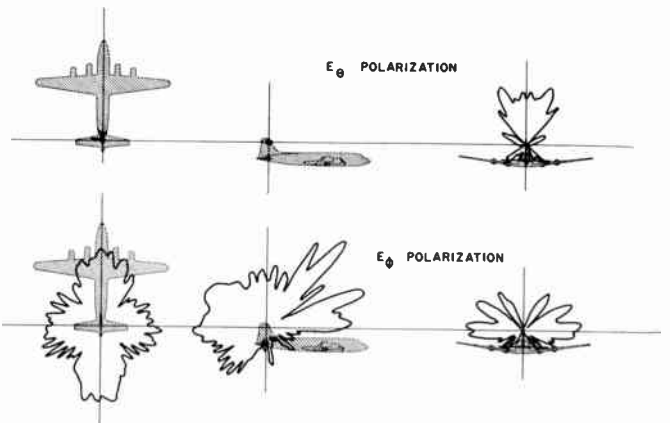
Fig. 27—Radiation patterns of a pair of E -fed cavity VOR antennas in the vertical stabilizer of a DC-6B aircraft.
