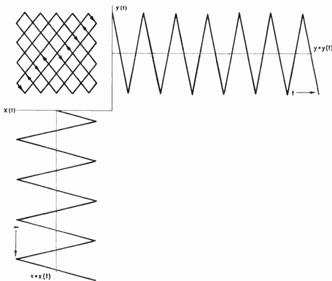
Fig. 2—Isotropic scan formed by triangular waves. Both the horizontal and vertical sweeps are triangular waves. In the present example there are five full waves in the vertical direction for every four full waves in the horizontal direction.
