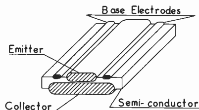
Fig. 5—Proposed electrode configuration for high power transistor.
