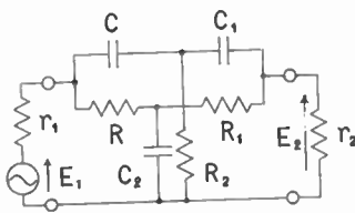
Fig. 1—Parallel- T rc network.
