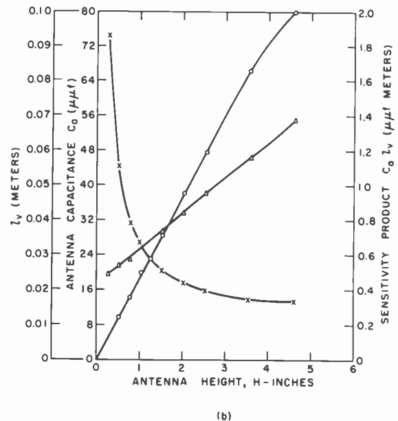
Fig. 5—Low-frequency design parameters, l_v and C_A for (a) flush antenna, and (b) low-silhouette protruding antenna.
