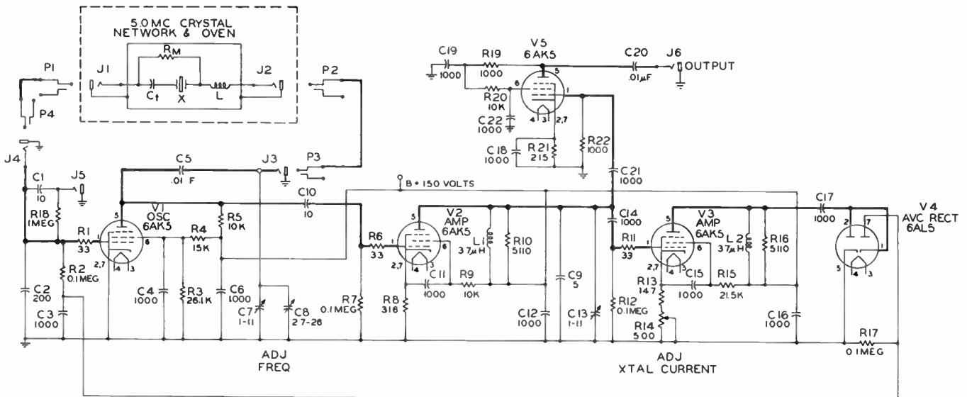
Fig. 4—Standard frequency oscillator circuit.
