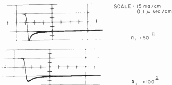
Fig. 5—Reverse recovery as a function of diode-loop resistance.
