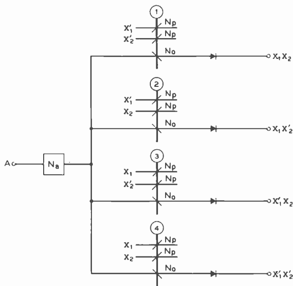
Fig. 13—A four-position AB-type switch.
