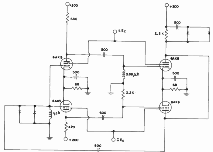
Fig. 8—An oscillator employing lead and lag networks.
