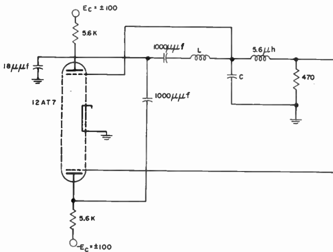
Fig. 6—A practical oscillator employing an artificial transmission line.
