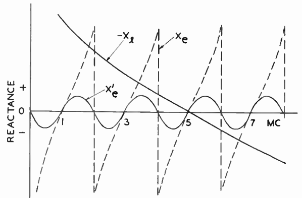
Fig. 3—Action of mode-suppression resistor.
