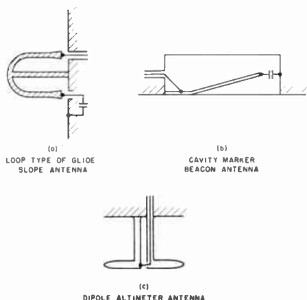
Fig. 20—Typical vhf aircraft antennas, (a) glide-slope antenna, (b) market beacon antenna, and (c) altimeter antenna.
