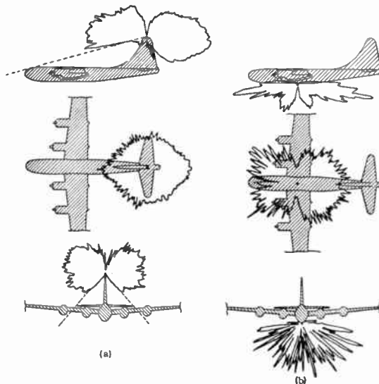
Fig. 21—Radiation patterns of 1000 mc stub antennas mounted (a) on the tip of the vertical stabilizer and (b) on the bottom centerline of a B-50 aircraft.
