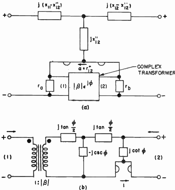
Fig. 5—Equivalent circuit for non-reciprocal two-port. (a) General equivalent circuit for two-port. (b) Complex transformer, |\beta|e^{j\phi} .
