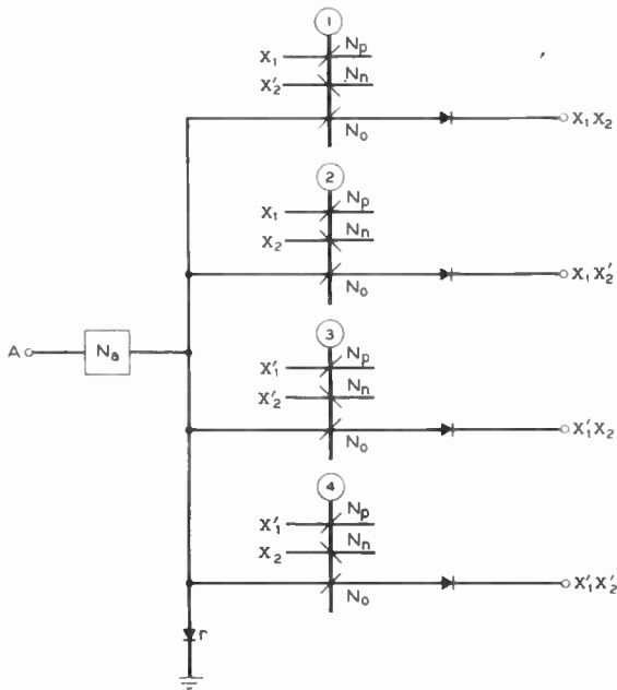
Fig. 10—A four-position AF-type switch.
