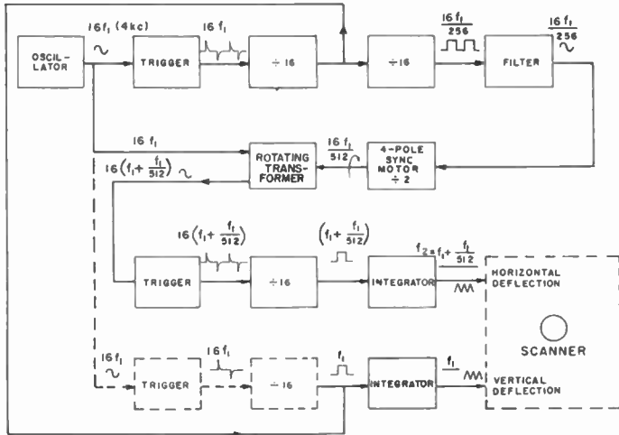
Fig. 4—Block diagram of the scan generator. The dotted line shows alternative connection
