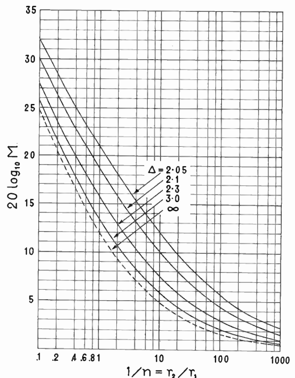
Fig. 2—Minimized loss at the extreme frequencies.
