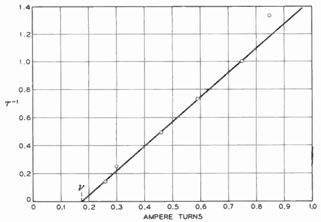
Fig. 3—Inverse switching time as a function of applied ampere-turns. A typical measurement.
