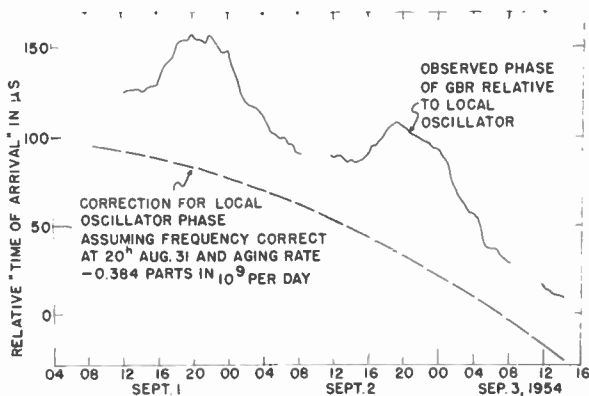
Fig. 6—Another example of the relative GBR phase, and of the presumed relative phase of the source, similar to Fig. 4.
