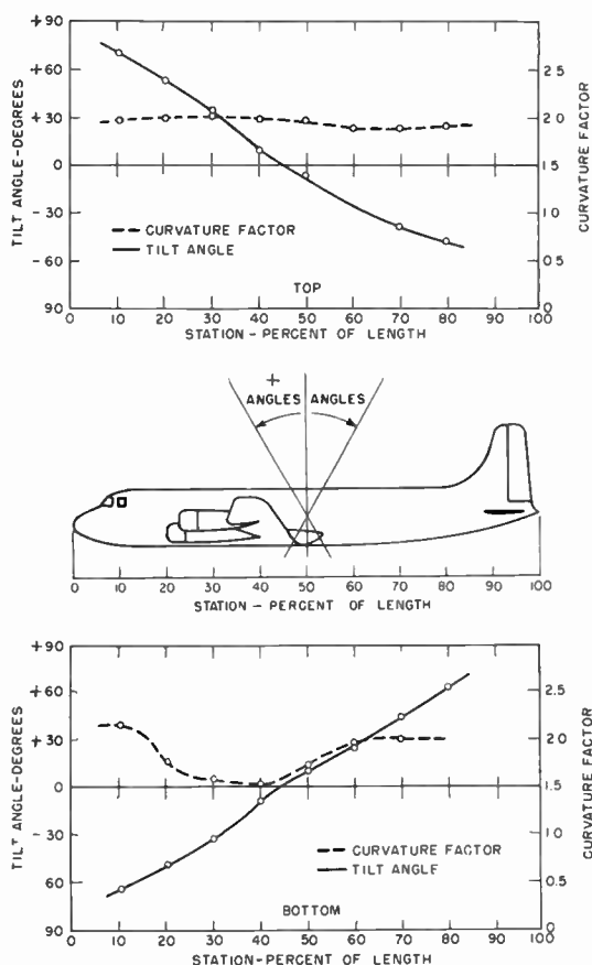
Fig. 4—Curvature factor and tilt angle survey data for DC-6 aircraft.
