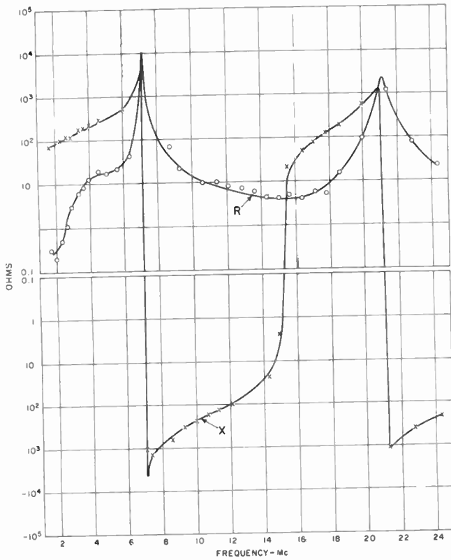
Fig. 16—Input impedance characteristic achieved with 30-foot shunt-feed element at inboard trailing edge of wing in 1049 Constellation aircraft.
