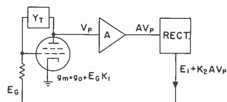
Fig. 2—Amplitude control circuit.
