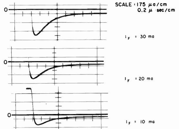
Fig. 9—Reverse recovery as a function of forward current using modified IBM circuit.
