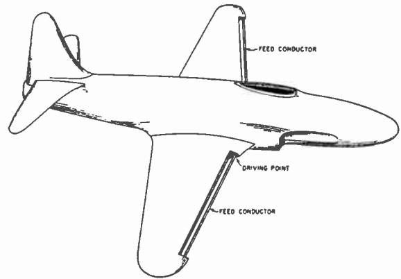
Fig. 15—Shunt feed technique utilizing leading edge of wing.
