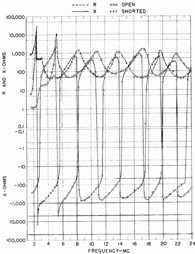
Fig. 9—Input impedance of 81-foot, open and shorted fixed-wire antennas on 1049 Constellation aircraft.
