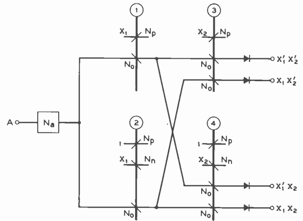
Fig. 14—Another four-position AB-type switch.
