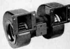
A15BD-8—115 Volt 60 cycle Double Blower. 46 CFM at .28" static pressure.
