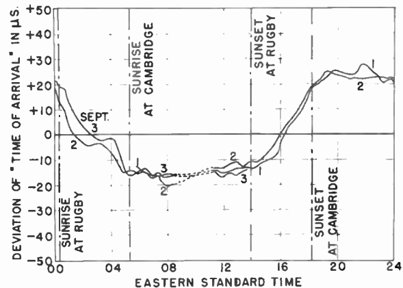
Fig. 7—The diurnal variations of GBR's transmission time for Sept. 1 to 3, 1954. Note that the anomaly of Fig. 5 is not present here.
