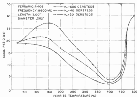
Fig. 2—Temperature dependence of the axial ratio in Ferramic A-106, with applied magnetic field as parameter.
