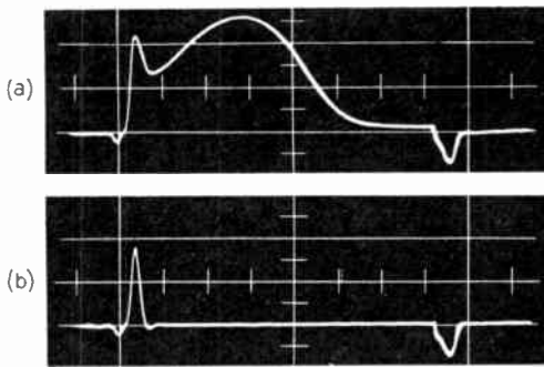
Fig. 2—Output voltage waveforms. (a) Switching voltage, (b) shuttle voltage.
