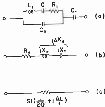
Fig. 6—Equivalent circuits of the crystal unit.
