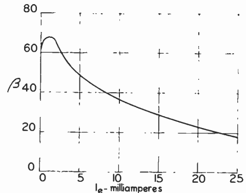
Fig. 2—Behavior of grounded emitter current gain, \beta , with I_e for typical low level transistor (after Webster, 2 Fig. 6).
