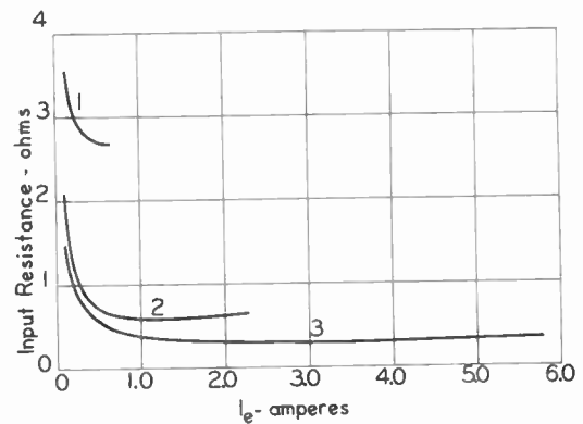
Fig. 8—Average grounded base input resistance V_e/I_e as a function of I_e for (1) X-78 standard power transistor, (2) single-bar unit, (3) double bar unit. All p-n-p types with V_c = -12 volts.
