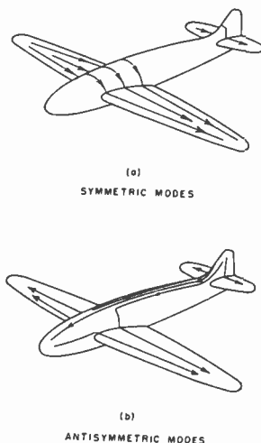
Fig. 8—Symmetric and antisymmetric modes of current on an airframe.
