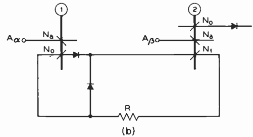
Fig. 7—T-type circuit with an input winding as the load. (1) One-diode configuration, (b) two-diode configuration.
