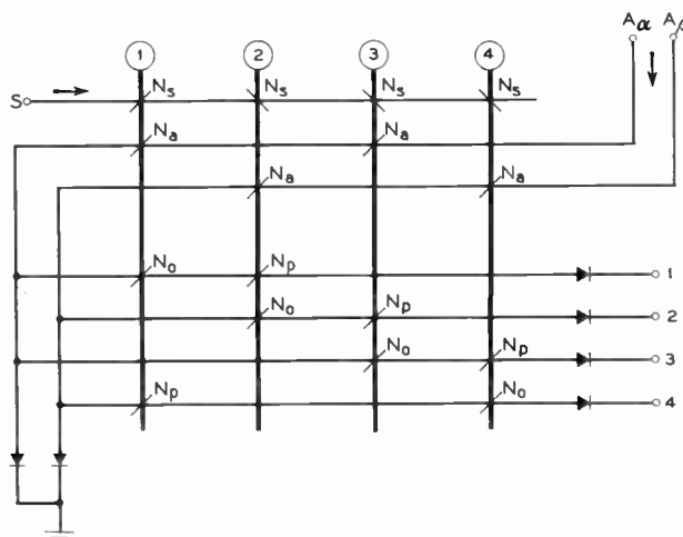
Fig. 17—Schematic of a two-phase AF-type stepping switch.
