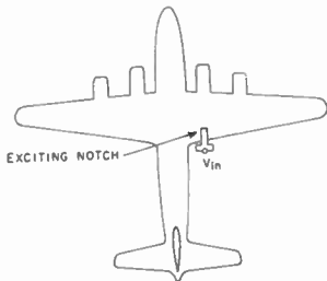
Fig. 17—Notch feed high-frequency antenna.
