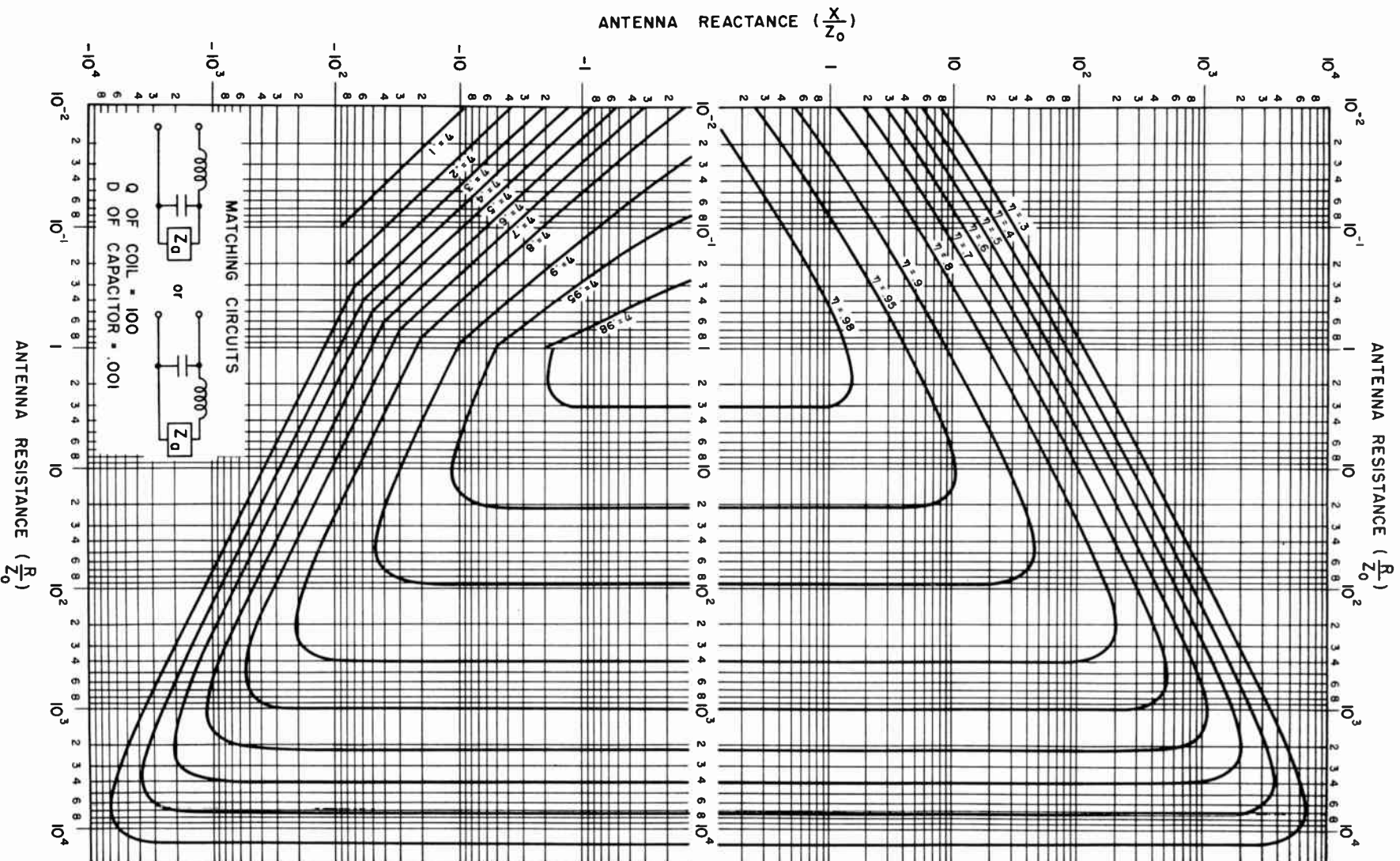
Fig. 18—Matching efficiency chart for L networks showing contours of equal power transfer efficiency on normalized R/Z_0 coordinate grid. Assumes coil Q of 100 and capacitor dissipation factor of 0.001.
