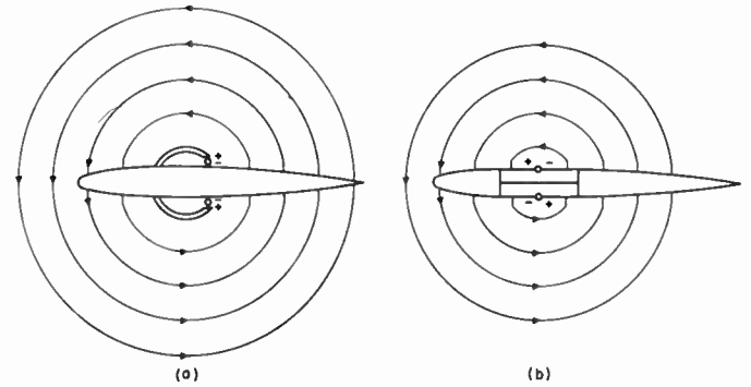
Fig. 26—Illustrating the technique for avoiding diffraction effects due to the vertical stabilizer by properly phasing a pair of symmetrically-located radiators.
