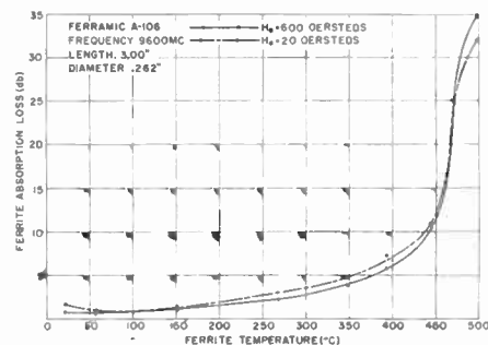
Fig. 3—Temperature dependence of the ferrite absorption loss in Ferramic A-106, with applied magnetic field as parameter.
