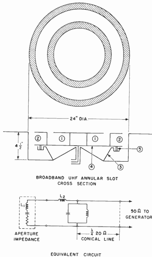
Fig. 29.—Annular slot antenna for the 225–400 mc band and equivalent circuit.
