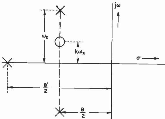
Fig. 3—Poles and zeros of the resonant-type oscillator.
