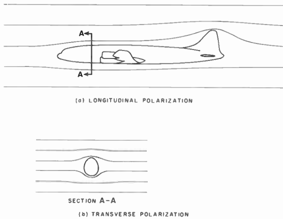
Fig. 6—Magnetic field distortion caused by conducting airframe for (a) longitudinal polarization, and (b) transverse polarization.
