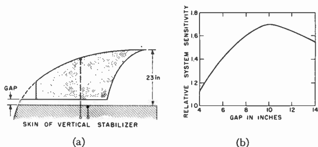
Fig. 3—Loran antenna on DC-6B aircraft: (a) physical configuration of antenna element, (b) dependence of system sensitivity on gap spacing.
