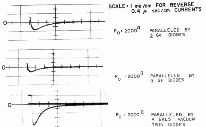
Fig. 7—Effect of by-pass diodes.
