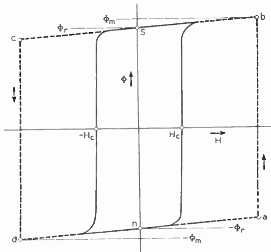
Fig. 1—A nearly rectangular hysteresis loop.
