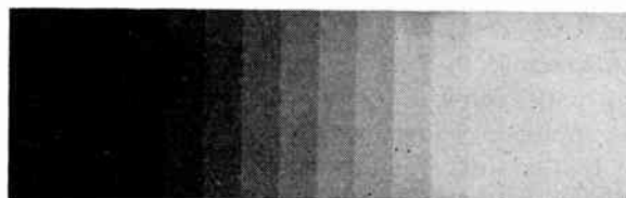
Fig. 1—Step tablet illustrating contour enhancement in the eye. Each step is a uniform shade of gray, although it appears lighter near the darker step and darker near the lighter one. The uniformity of each area can be checked by masking all steps except one.
