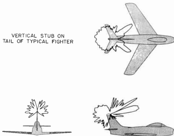
Fig. 22—Radiation patterns of a 300 mc stub antenna on the stabilizer tip of a fighter aircraft.
