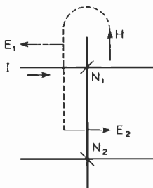
Fig. 4—Mirror symbol notation for schematics of magnetic core circuits.
