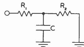
Fig. 9—Electrical analog for thermal impedance R .
