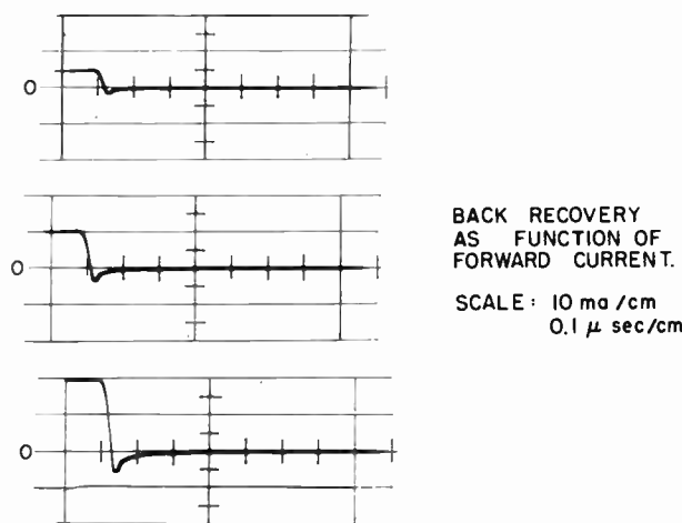
Fig. 3—Reverse recovery as a function of forward current.
