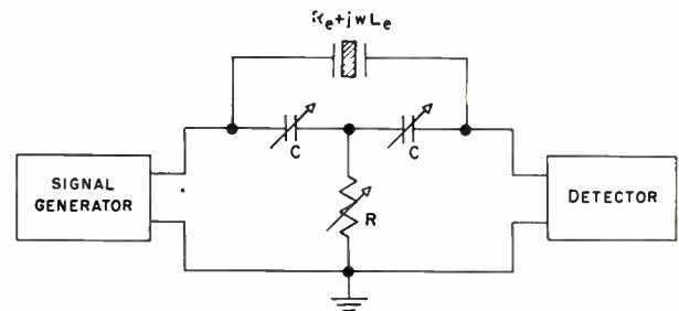
Fig. 15—Bridged T-network.
