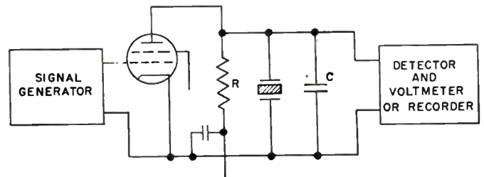
Fig. 7—Anti-resonance measuring circuit.
