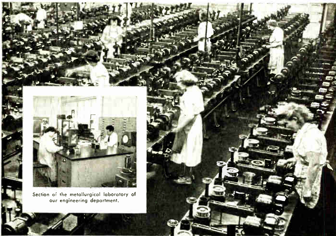
General view of Sylvania tungsten wire drawing department at our Towanda, Pa. plant.
