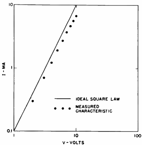
Fig. 4—Volt-ampere characteristic of square-law rectifier (log-log coordinates).
