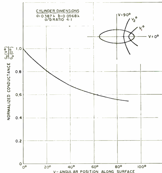
Fig. 5—Effect of position of axial slot on the radiation conductance.
