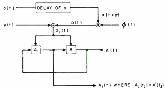
Fig. 10—Block diagram of the phase-bistable flip-flop.
