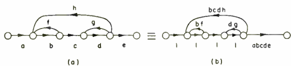
Fig. 30—Normalization.
