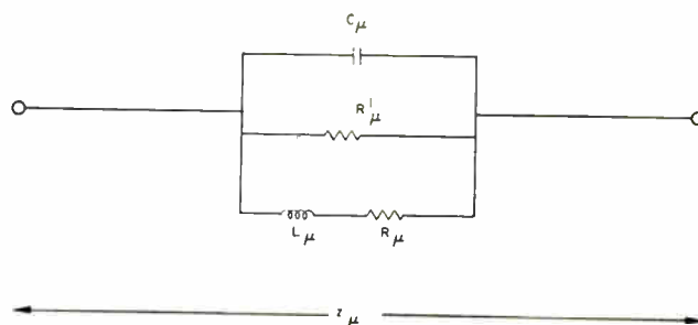
Fig. 5—Network realization of pair of complex conjugate poles where z_\mu is given by (12).
