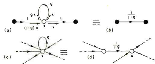
Fig. 16—Replacement of a self-loop by a branch.
