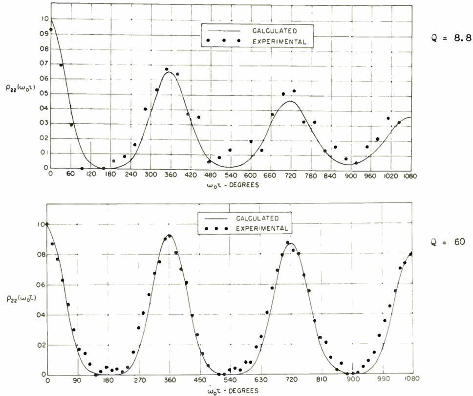
Fig. 12—Normalized output autocorrelation functions \rho_{22}(\omega_0\tau) for square-law rectifier with filtered noise input.
