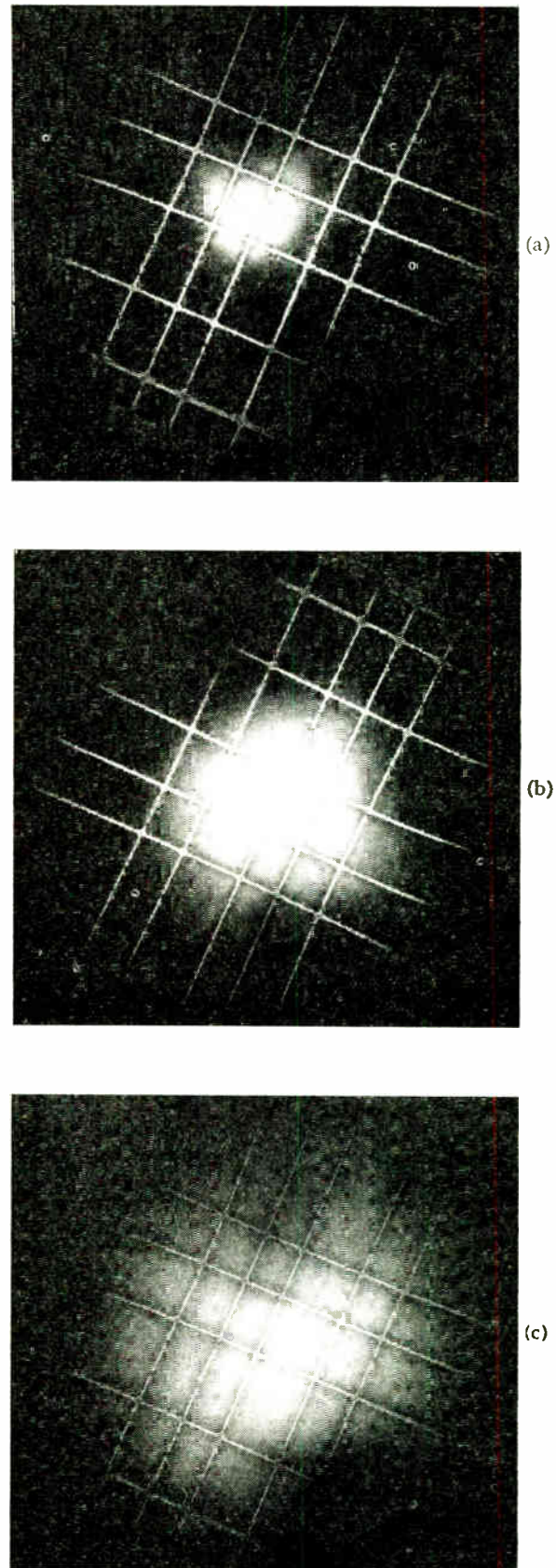
Fig. 4—Viewing-screen photographs of an early model of the direct-viewing memory tube with a negative background and five vertical and five horizontal positive lines written. Note appearance of the negative background for three different settings of the contrast control V_b - V_n . (a) 0 volts; (b) 100 volts; (c) 200 volts.
