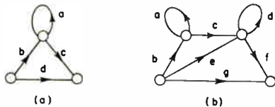
Fig. 17—Residues having first-index feedback units.
