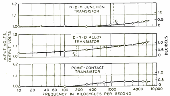
Fig. 12—Measured values of ratio of input to output voltage as function of frequency. XY transmission. R_x = 5620 ohms.
