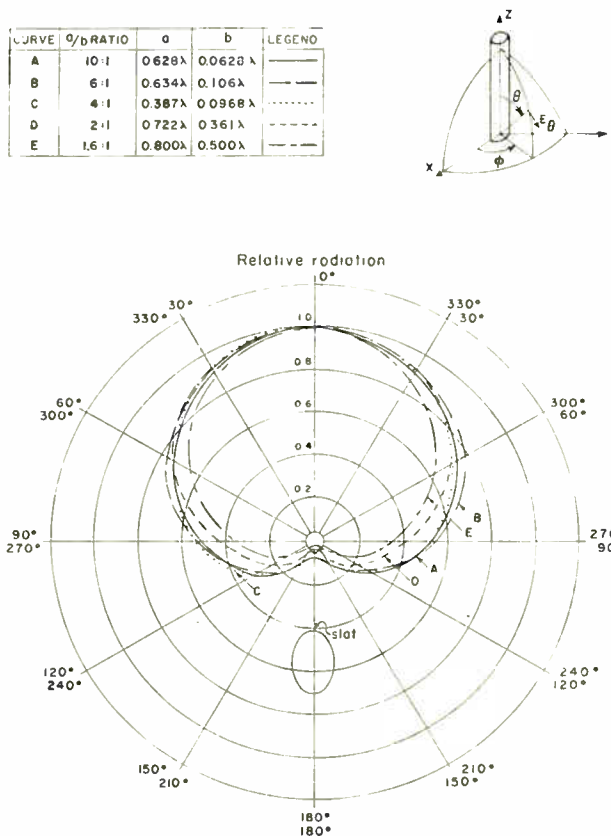
Fig. 3— E_\theta field from \lambda/8 transverse slot in elliptic cylinder. Field in horizontal plane \theta = \pi/2 .
