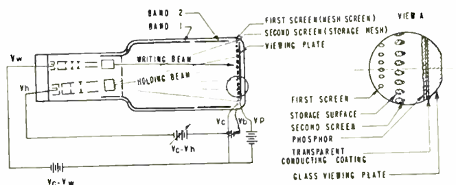
Fig. 1—Diagram of the direct-viewing memory tube.
