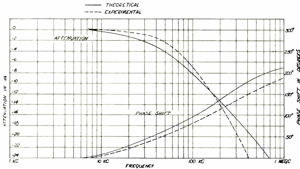
Fig. 7—Experimental and theoretical phase and attenuation characteristics.
