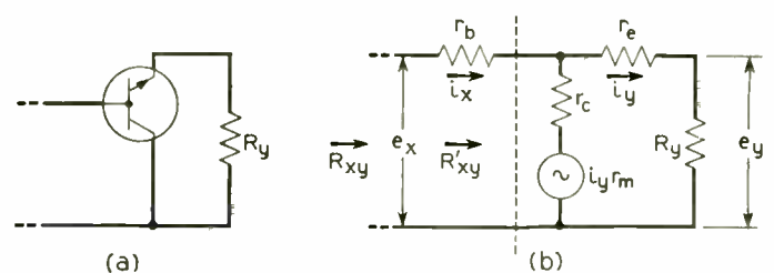
Fig. 1—Common-collector amplifier transmitting in the XY direction: (a) schematic, and (b) equivalent circuit.
