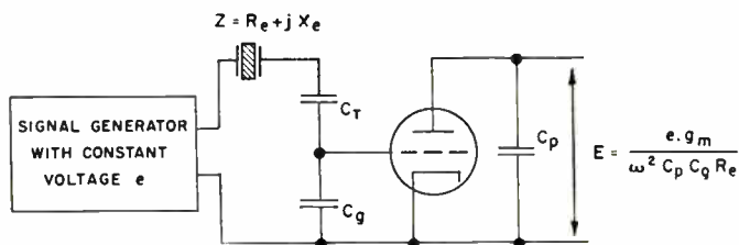
Fig. 12—The performance index (PI) meter circuit.
