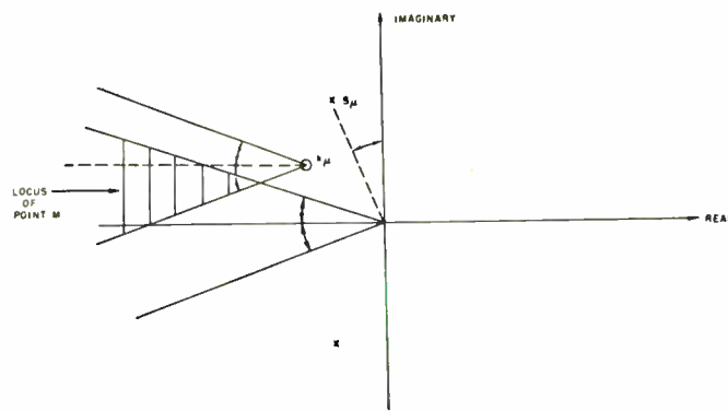
(b) Locus of M (crosshatched portion) for \alpha_{\mu} negative.
