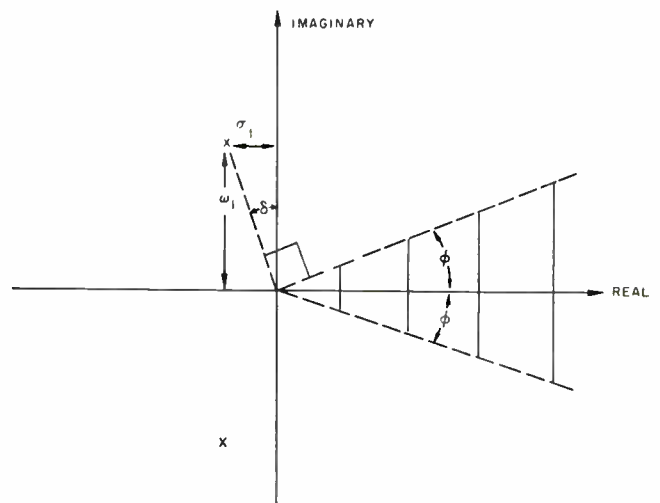
Fig. 2—Geometrical illustration of pole and residue relationship.
