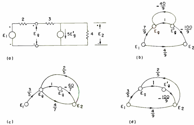
Fig. 32—An amplifier with grid-to-plate impedance.
