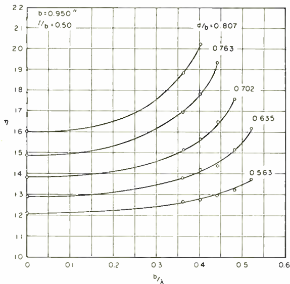
Fig. 7—Index of refraction of square obstacles on 0.005-inch polystyrene sheets spaced by polyfoam, l/b=0.50 .
