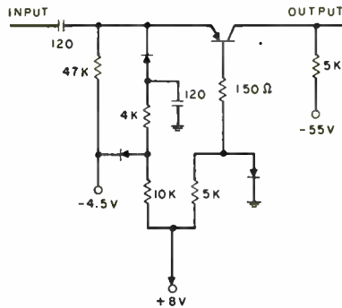
Fig. 5—Circuit diagram of the one-shot multivibrator.
