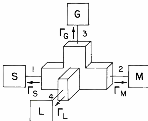
Fig. 4—Magic T comparison.
