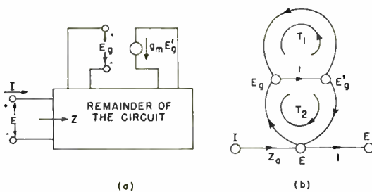
Fig. 33—The circuit and graph for terminal impedance formulation.
