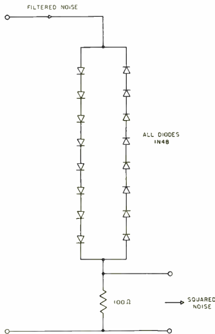
Fig. 8—Circuit for squaring input voltage.
