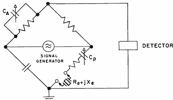
Fig. 13—Radio frequency bridge. R_e is balanced by C_A , X_e by C_p .
