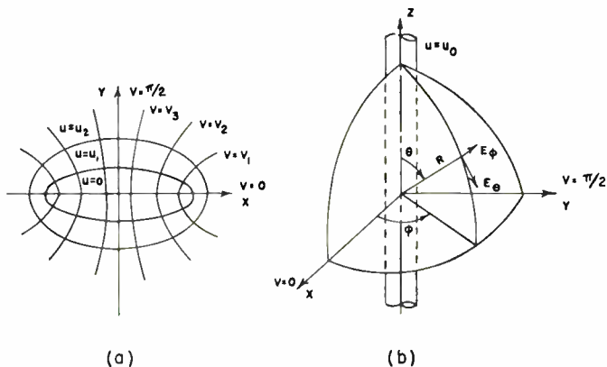
Fig. 1—Elliptic cylinder co-ordinate system.
