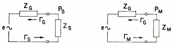
Fig. 1—Alternate connection to stable source.
