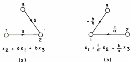
Fig. 27—Branch inversion in a linear graph.
