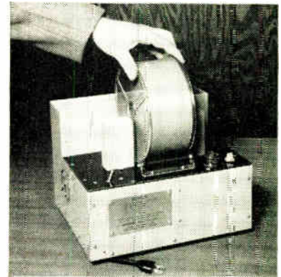
Erase the 24-hour tape in just 20 seconds — simply by rotating the reel in the SoundScriber Tape Demagnetizer!
