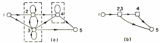
Fig. 9—The condensation of a flow graph.
