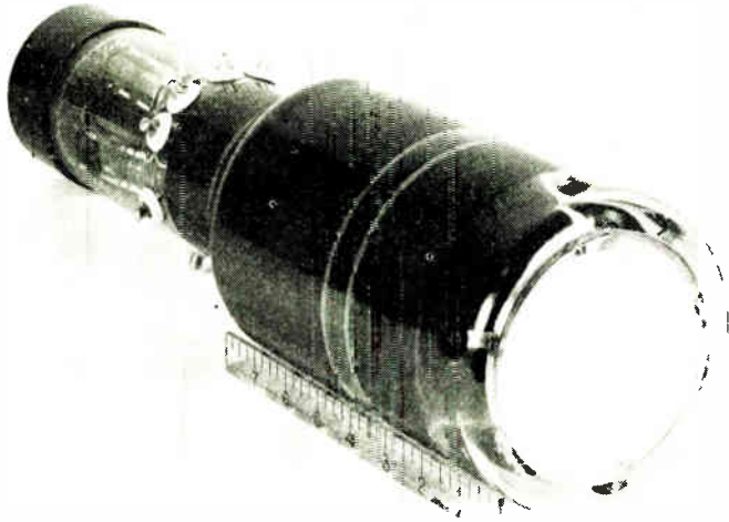
Fig. 2—Direct-viewing memory tube with electrostatically focused electron guns. Scale is in inches.
