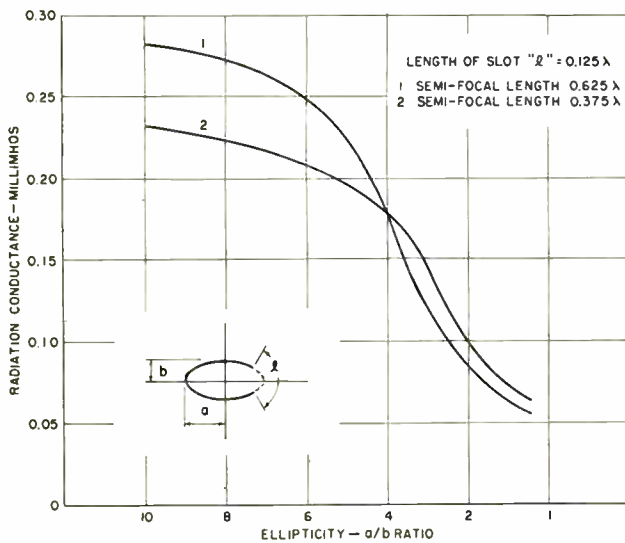
Fig. 6—Radiation conductance of cylinder of transverse slot in elliptical cylinder.
