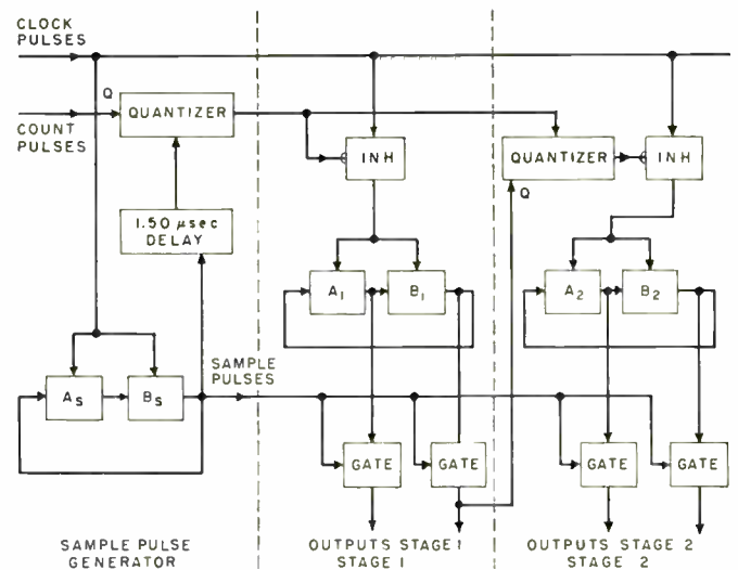
Fig. 8—Block diagram of the two-stage binary counter.
