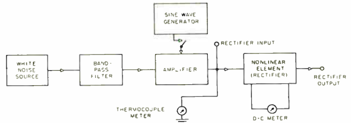
Fig. 2—Block-diagram representation of circuit.
