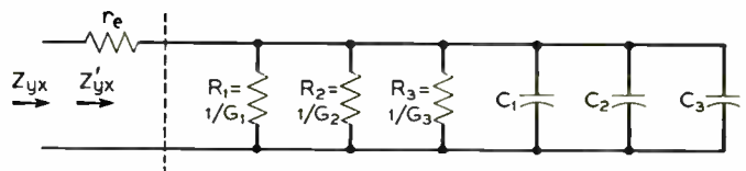
Fig. 8—Equivalent circuit for input impedance of common-collector amplifier. YX transmission.
