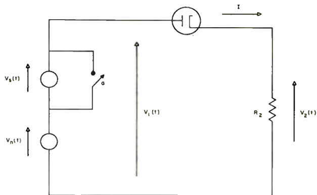
Fig. 5—Simplified circuit diagram with V_n = filtered random noise of center frequency \omega_0 , and V_s = P \cos \omega_0 t .
