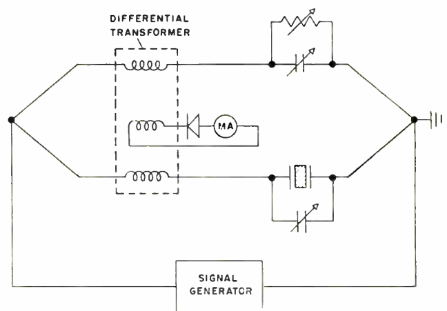
Fig. 16—Differential bridge.
