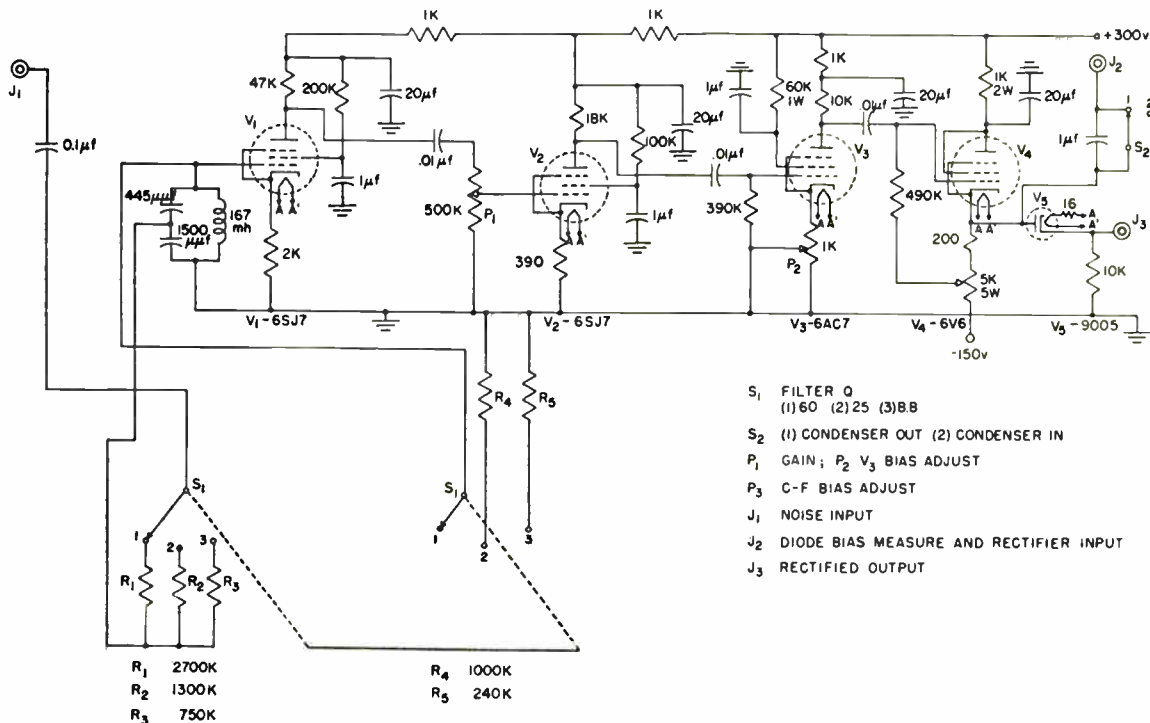
Fig. 3—Circuit diagram of amplifier including band-pass filter and nonlinear element.
