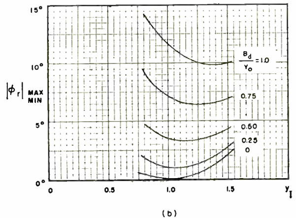
Fig. 4—Phase-shift errors. (a) Residual transmission-coefficient phase shift after subtracting phase shift of an isolated sheet, B_d = B/2 ; (b) Extreme values of phase-shift deviation due to internal reflections.
