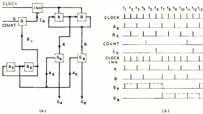
Fig. 4—Method of inhibiting clock pulses accomplished by count pulses occurring at random intervals.
