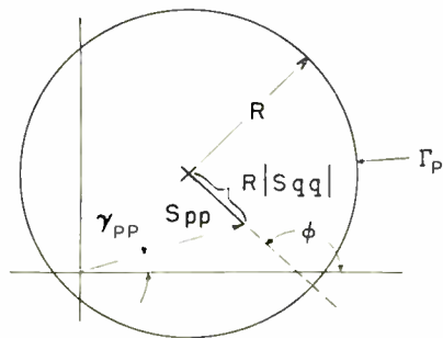
Fig. 11—Reflection coefficient circle.
