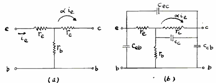
Fig. 1—AC equivalent circuit of a transistor neglecting diffusion effects of the carriers.
