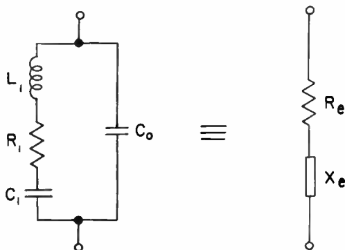
Fig. 1—Equivalent circuits of a piezoelectric vibrator.
