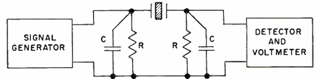
Fig. 6—Transmission measuring circuit.
