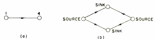
Fig. 6—Residual forms of a cascade graph.
