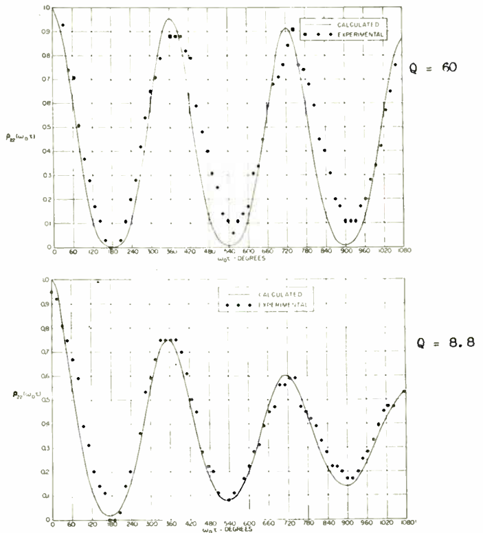
Fig. 10—Normalized output autocorrelation functions \rho_{22}(\omega_0\tau) for linear rectifier with a filtered noise input.
