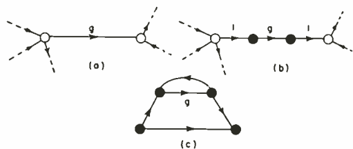
Fig. 25—The graph gain as a function of a particular branch gain.
