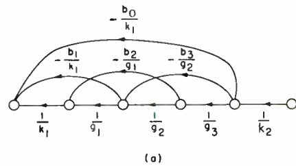
Fig. 28—The result of path inversion in Fig. 20(a).
