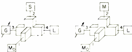
Fig. 6—Alternate connection to a magic T .
