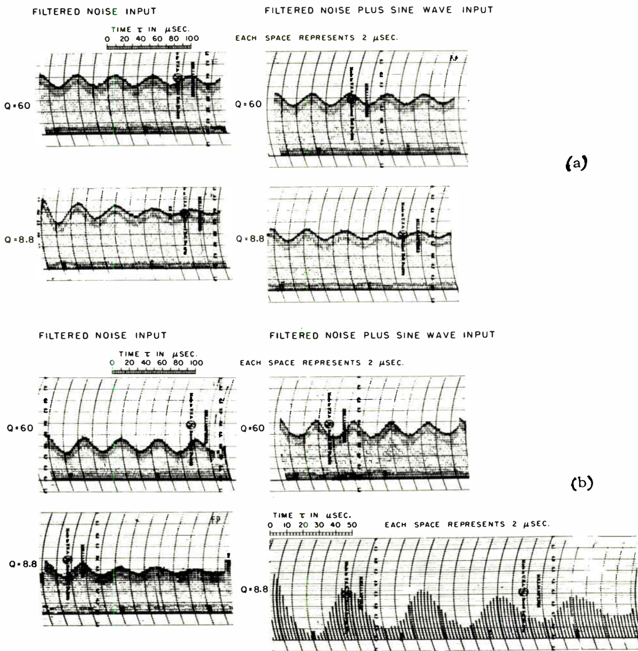
Fig. 7—Autocorrelation functions as recorded by correlator: (a) input autocorrelation functions, and (b) output auto correlation functions for linear rectifier.
