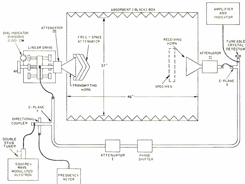
Fig. 1—Dielectric apparatus used for index-of-refraction measurements.
