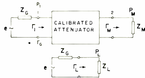
Fig. 7—Use of calibrated attenuator.
