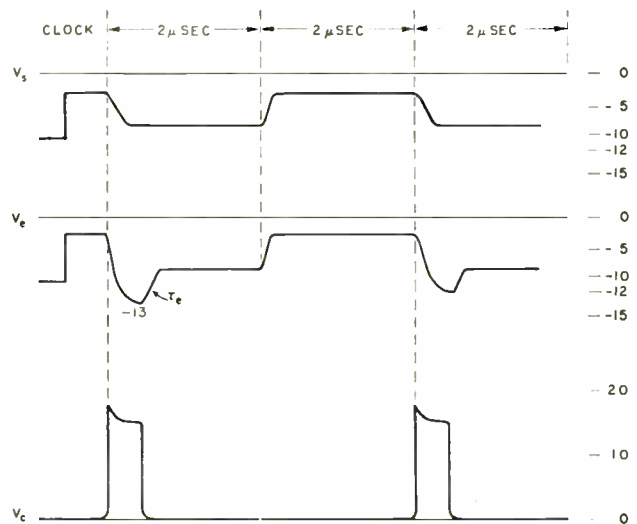
Fig. 6b—Detailed operation of the commutating-ring circuit.
