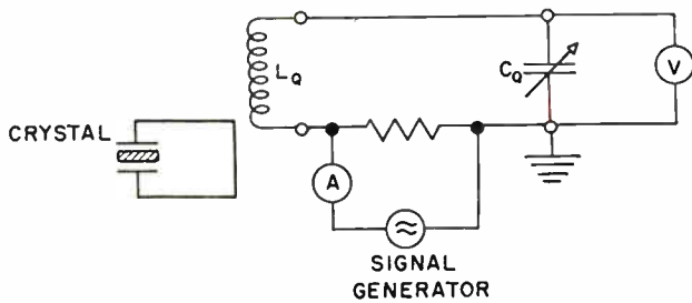
Fig. 4—Measurement of the characteristic frequency f_m (at minimum impedance) in the Q -meter.
