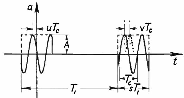
Fig. 2—Example of a pulse series.
