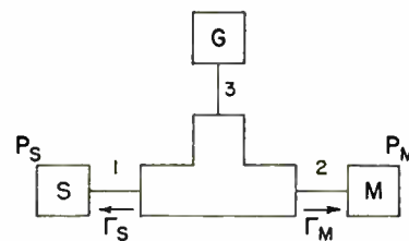
Fig. 2—T-junction comparison.
