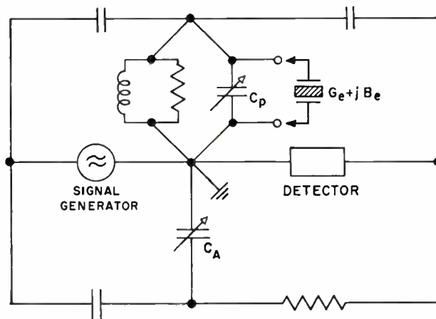
Fig. 14—Twin-T impedance measuring circuit. The conductance G_e is balanced by C_A , the susceptance B_e by C_p
