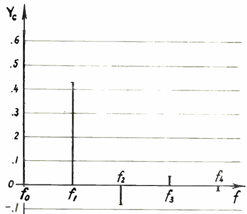
Fig. 11—Ordinary presentation of the spectrum of Fig. 10.
