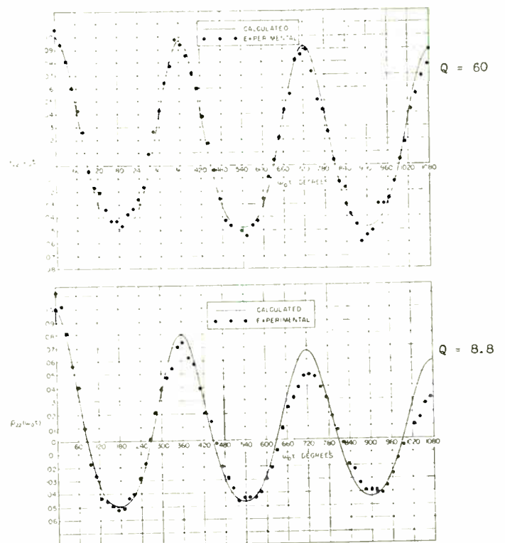
Fig. 11—Normalized output autocorrelation functions \rho_{22}(\omega_0\tau) for linear rectifier with a filtered noise plus sine wave input, where x = sine wave power/noise power = 1.
