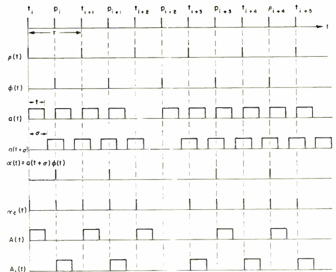
Fig. 9—The timing sequence of the two-stage binary counter.
