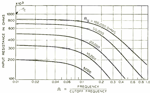
Fig. 6—Input resistance (XY transmission) for transistor having \alpha_0 = 0.98 , r_c = 1 megohm, f_c = 2 megacycles and c_c = 5 mmf.
