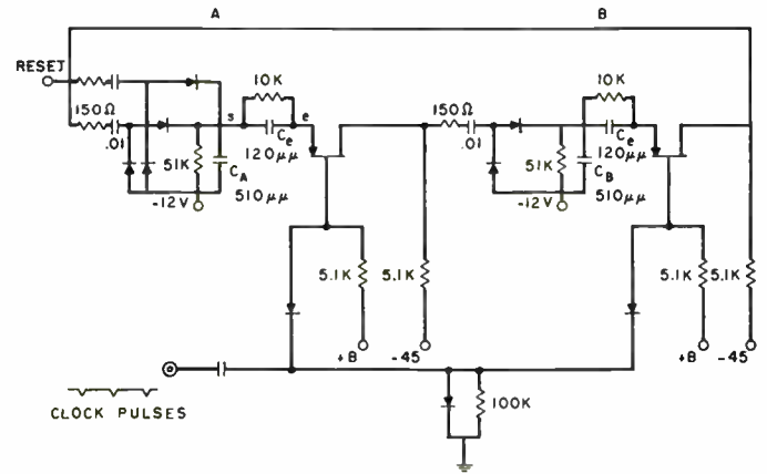
Fig. 6a—Circuit diagram of the commutating ring.
