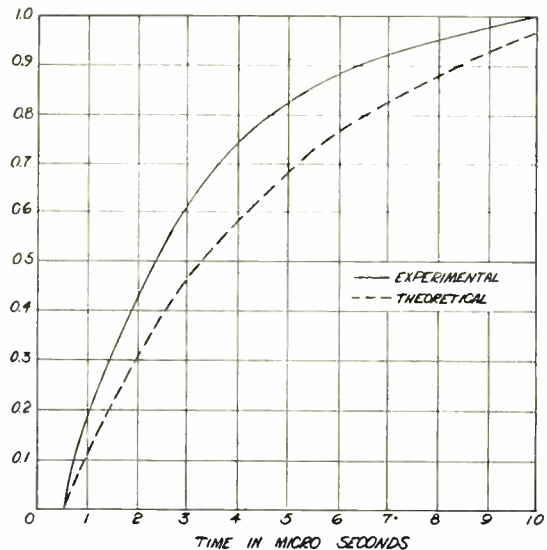
Fig. 8—Theoretical and experimental transient response.
