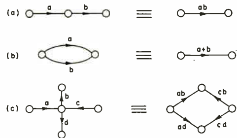
Fig. 13—Elementary transformations.
