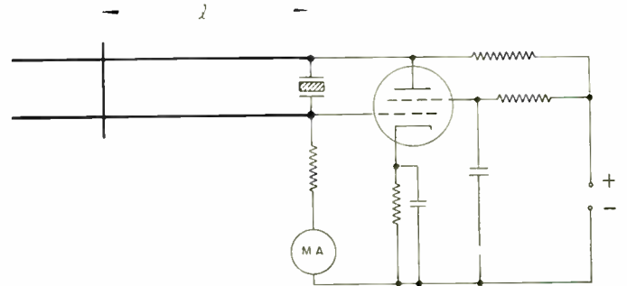
Fig. 18—Transmission-line reactance meter.
