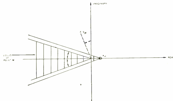
(c) Locus of M (crosshatched portion) for \beta_{\mu} = 0 and \alpha_{\mu} positive
