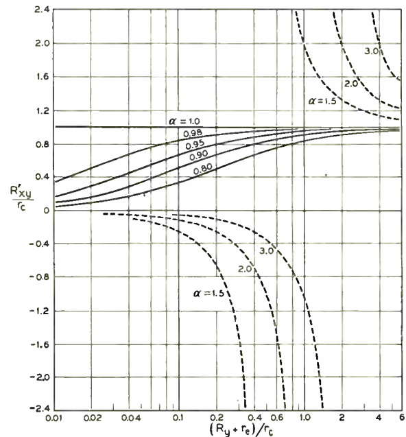
Fig. 3—Variation of input resistance as a function of load resistance— XY transmission.
