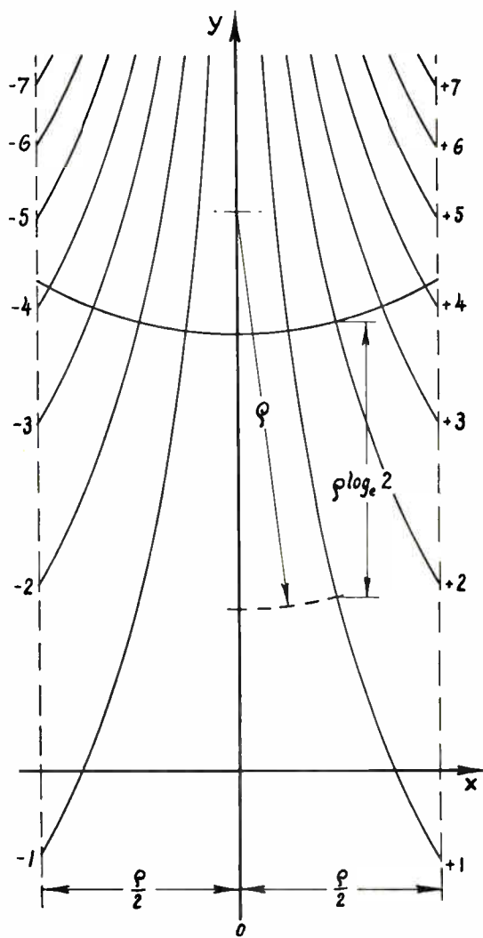
Fig. 6—The family of convergent logarithmic cycloids.
