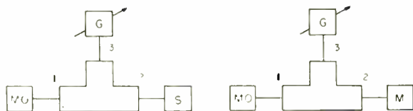
Fig. 3—Alternate connection to a T junction.
