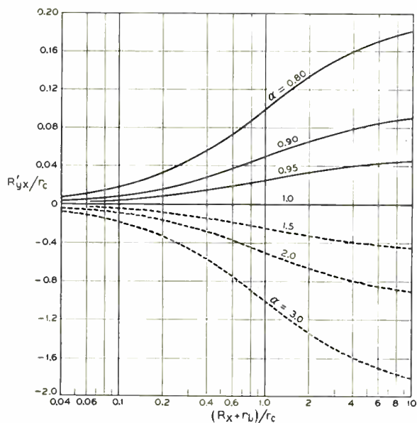
Fig. 4—Variation of input resistance as a function of load resistance —YX transmission. Note that scale for R'_{yx}/r_c is different for positive and negative values.
