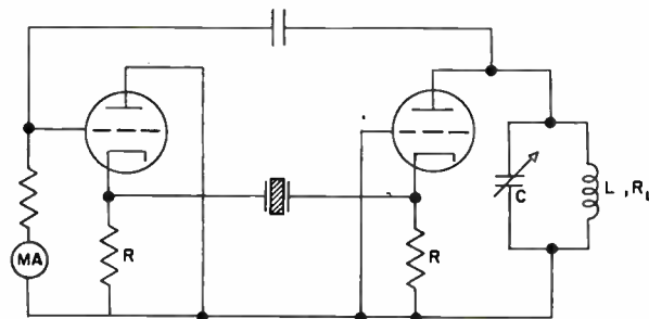
Fig. 10—Butler circuit.
