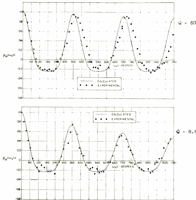
Fig. 13—Normalized output autocorrelation functions \rho_{22}(\omega_0\tau) for square-law rectifier with filtered noise plus sine wave input, where x = \text{sine wave power/noise power} = 1 .
