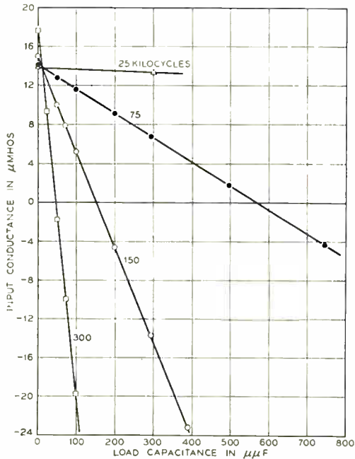
Fig. 13—Input conductance as a function of load capacitance. XY transmission. R_v = 10,000 ohms.
