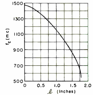
Fig. 2—Cutoff frequency vs. ridge depth.
