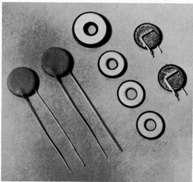
(Victory Engineering Corp.) Fig. 901-b. Photo shows varistors in different stages of production.
