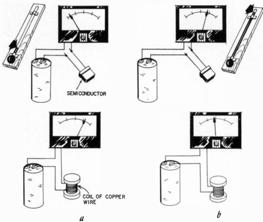
Fig. 201. At a low temperature (a) the semiconductor conducts very little and the conductor freely. When the temperature is raised (b) the semiconductor conducts much more and the conductor slightly less. The temperature sensitivity of a semiconductor can have a useful application, as in the germanium resistance thermometer shown in the photo. (Courtesy Bell Telephone Laboratories)
