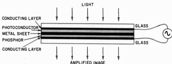
Fig. 909. Section of panel combining the photoconductive cell in Fig. 908 with the electroluminescent part.
