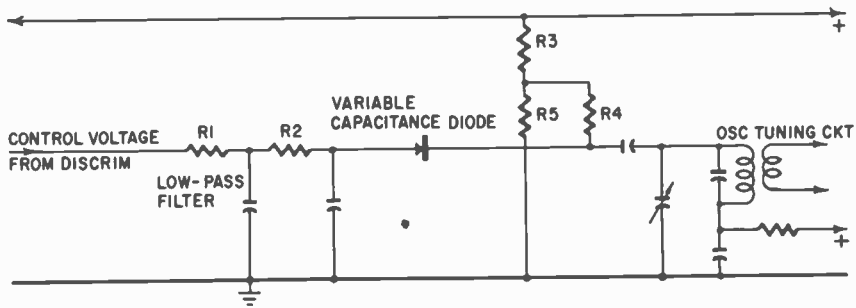
Fig. 915. Afc circuit, using a semiconductor diode as the variable reactance element.
