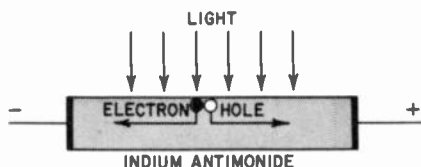
Fig. 812. Showing the principle of the photoelectromagnetic type of cell, in which a magnetic field must be provided to act at right angles to the light and to the electric current resulting. In this case the direction of the field is into the paper.
