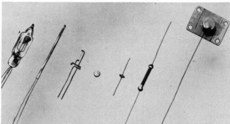
Fig.-902. Two uses of thermistors in a tube heater circuit. The photo shows various types.
