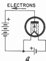
Fig. 505. In a diode tube, a positive charge on the anode attracts electrons across and sets up a current (a); negative repels and holds them back, so no current (b).
