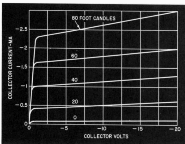
Fig. 800. Phototransistor characteristic curves, which should be compared with Fig. 705.
