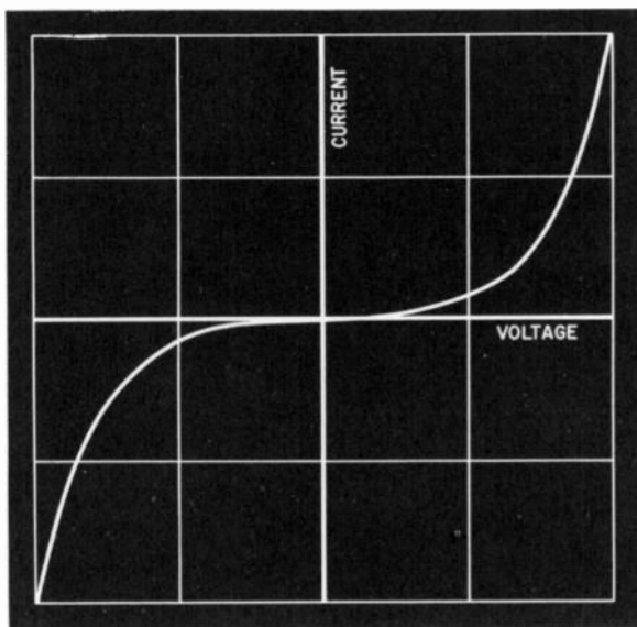
Fig. 901-a. Typical shape of varistor current/voltage characteristic curve.
