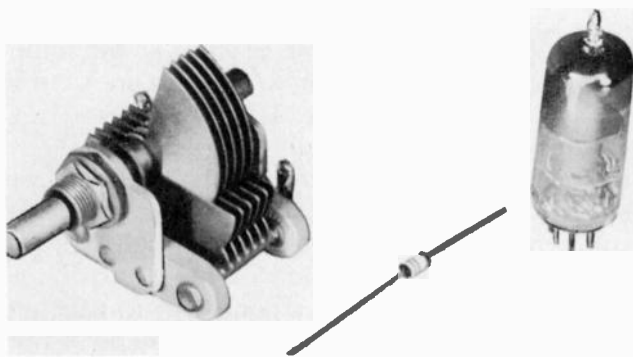
Fig. 916. The capacitance of this little semiconductor, the size of a \frac{1}{4} -watt resistor, varies with the voltage applied to it.
