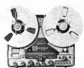
MAGNECORD MODEL 1048 Professional 2 channel (stereo) recorder/reproducer for use in main studio, production studio or conference recording. (10½" reel capacity) Model 1048 is available in ½- or ¼-track.
