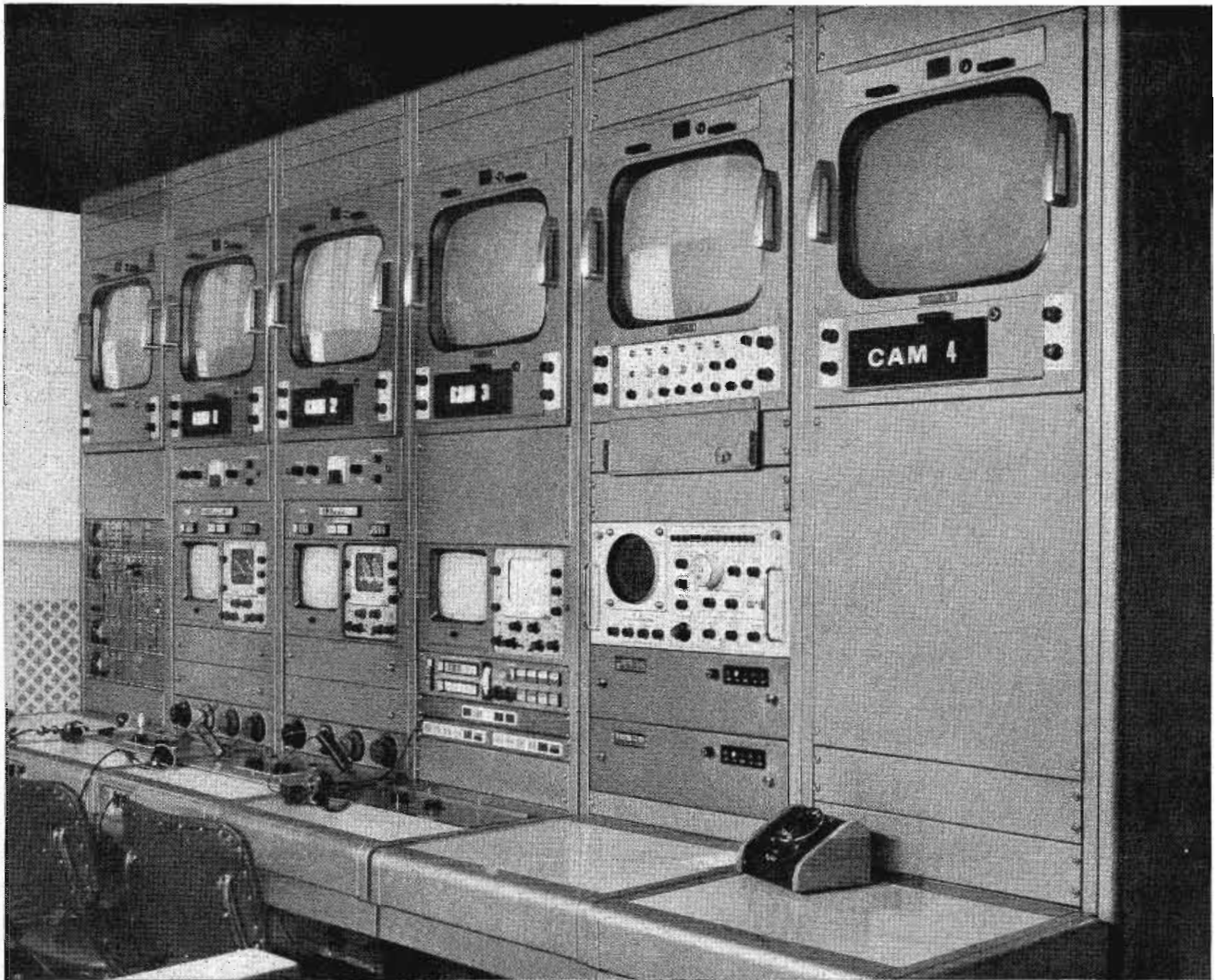
Photo of EMCOR I series cabinetry, courtesy of General Electric Co.
