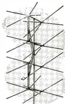
MODEL 8X-TV Super Hi-Gain 4 Bay Stacked Array
