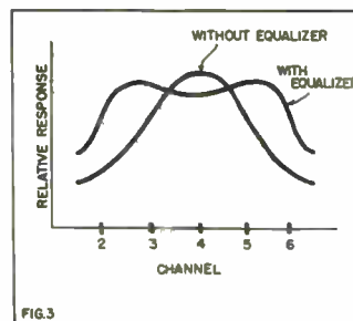
Fig. 3 Relative response of short dipole over channels 2 thru 6, with & without equalizer
