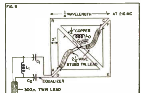
Fig. 9 Motorola's built-in antenna
