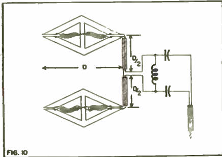
Fig. 10 Stacked Motorola antenna
