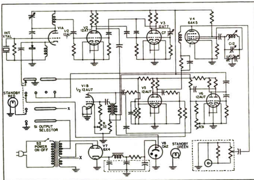
Fig. 1 Simplified schematic diagram of Hickok's Linearity Pattern Signal Generator
