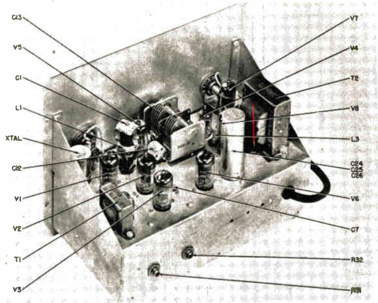
Chassis view of the instrument. Schematic below shows function of components
