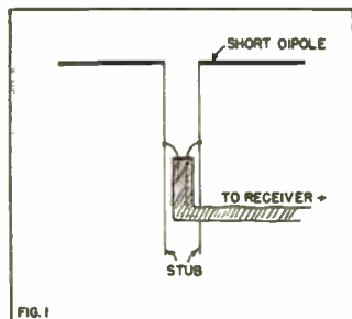
Fig. 1 Increasing efficiency of short dipole through use of high selectivity tuning network
