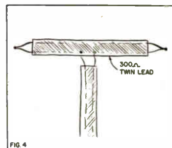
Fig. 4 Folded dipole arrangement used for some built-in antennas (RCA, Emerson, et. al.)
