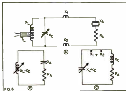
Fig. 8 Equivalent Circuit of Philco's antenna
