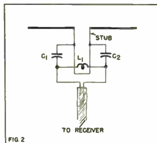
Fig. 2 An equalizer added to the tuning stub tunes dipole for broadband response (about 30 Mc)
