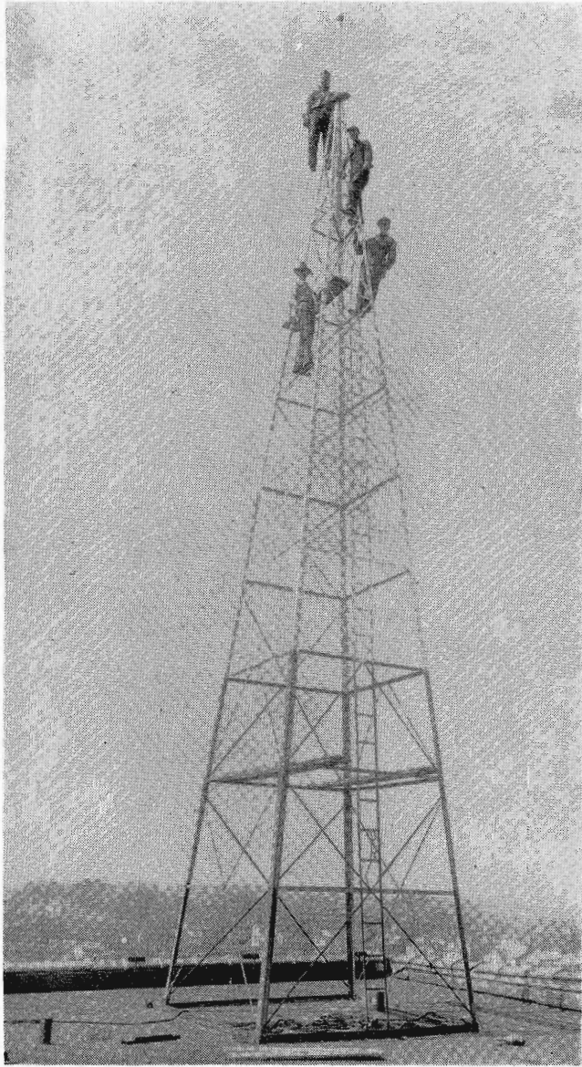
One of the two fifty foot windmill towers supporting WBTM's 'T' type antenna back in the thirties. This was a far cry from WBTM's three tower directional array of antennas as used today.
