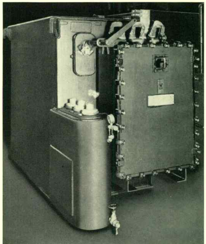
A portable sealed-tank dry-type transformer in service in a coal mine is shown above. Below is an external view of the first 500-kva, 13-kv submersible dry-type network transformer, installed in 1943. The high-voltage, single-conductor cables enter the transformer through a terminal chamber mounted on one end of the tank.
