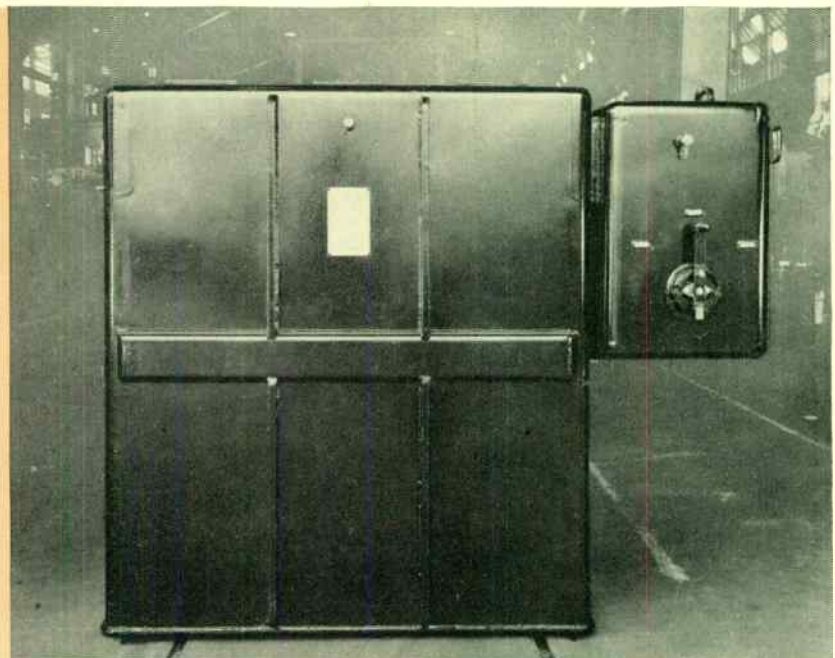
The complete submersible dry-type transformer, rated 500 kva, 3 phase, 11 800/216 volts, and its core and coils.
