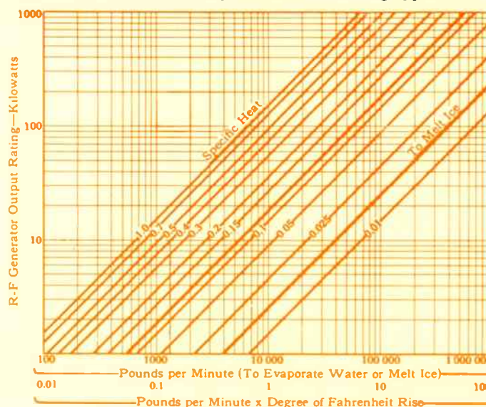
Fig. 2—R-f generator rating for dielectric-heating applications.
