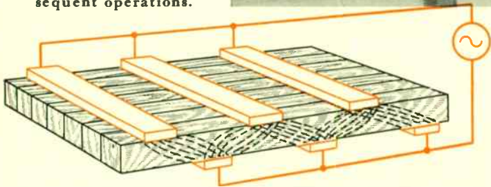
Fig. 4—Staggered arrangement of electrodes produces zigzag glue cure pattern, for partial curing of glue-line area. Area cured immediately is approximately one third of total glue-line area, providing sufficient strength for subsequent operations.
