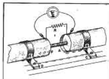
Figure 2 Alternate current patterns which appear around a bad joint and result in the radiation of noise.
