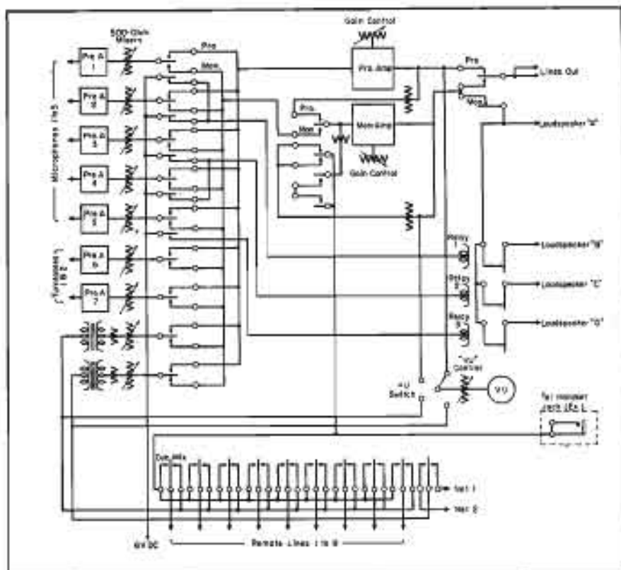
Figure 4 Block diagram of the console used at WGNR.
