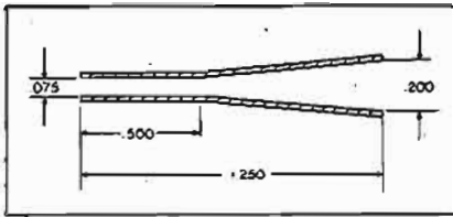
Figure 2 Dimensions of the D_3D_4 deflecting plates of the wide band crt .
