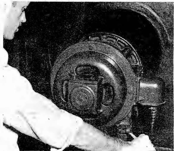
Figure 7 Tightening the motor foot bolts to guard against vibration. This step, which might appear minor, is a very important one, for vibration can throw plenty of punishment on the motor and decrease its life considerably.
