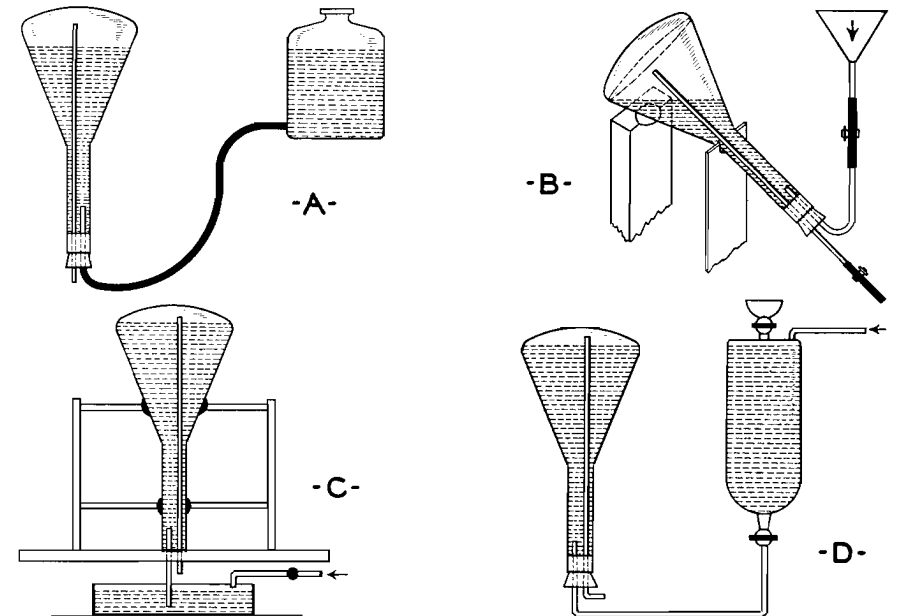
Fig. 3. Setups used in applying colloidal graphite dispersions. (3D, H. W. Weinhart, U. S. Patent No. 2096416.)
