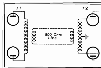
Below: Fig. 1. Illustrating an amplifier with a 500-ohm output winding driving a Class B audio stage.
