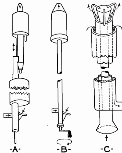
Fig. 2. Types of mechanical devices used in applying fluorescent powders.
