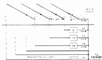
Fig. 2. Showing directive antennas and phase-shifting networks.
