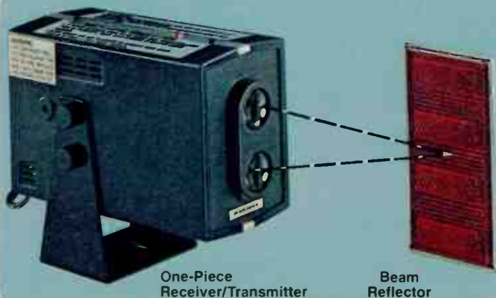
Beam Reflector
