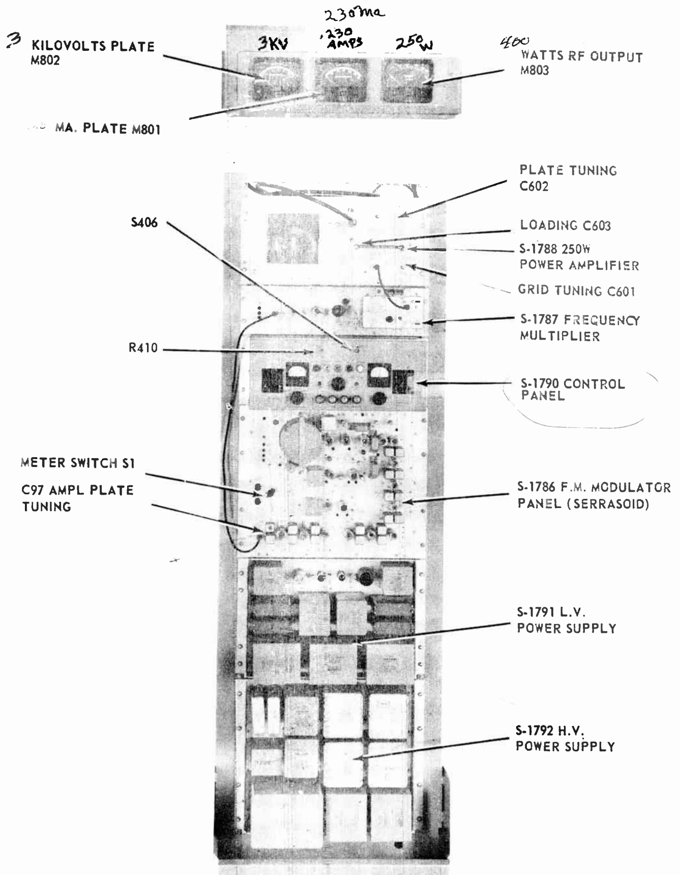
Figure 5-1 Type 930 F.M. Multiplex Transmitter, front view
