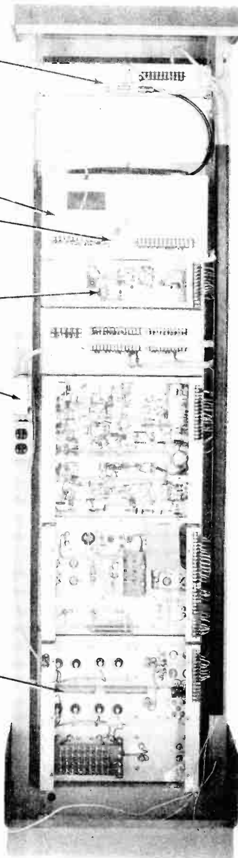
Figure 5-2 Type 930 F.M. Multiplex Transmitter, rear view
