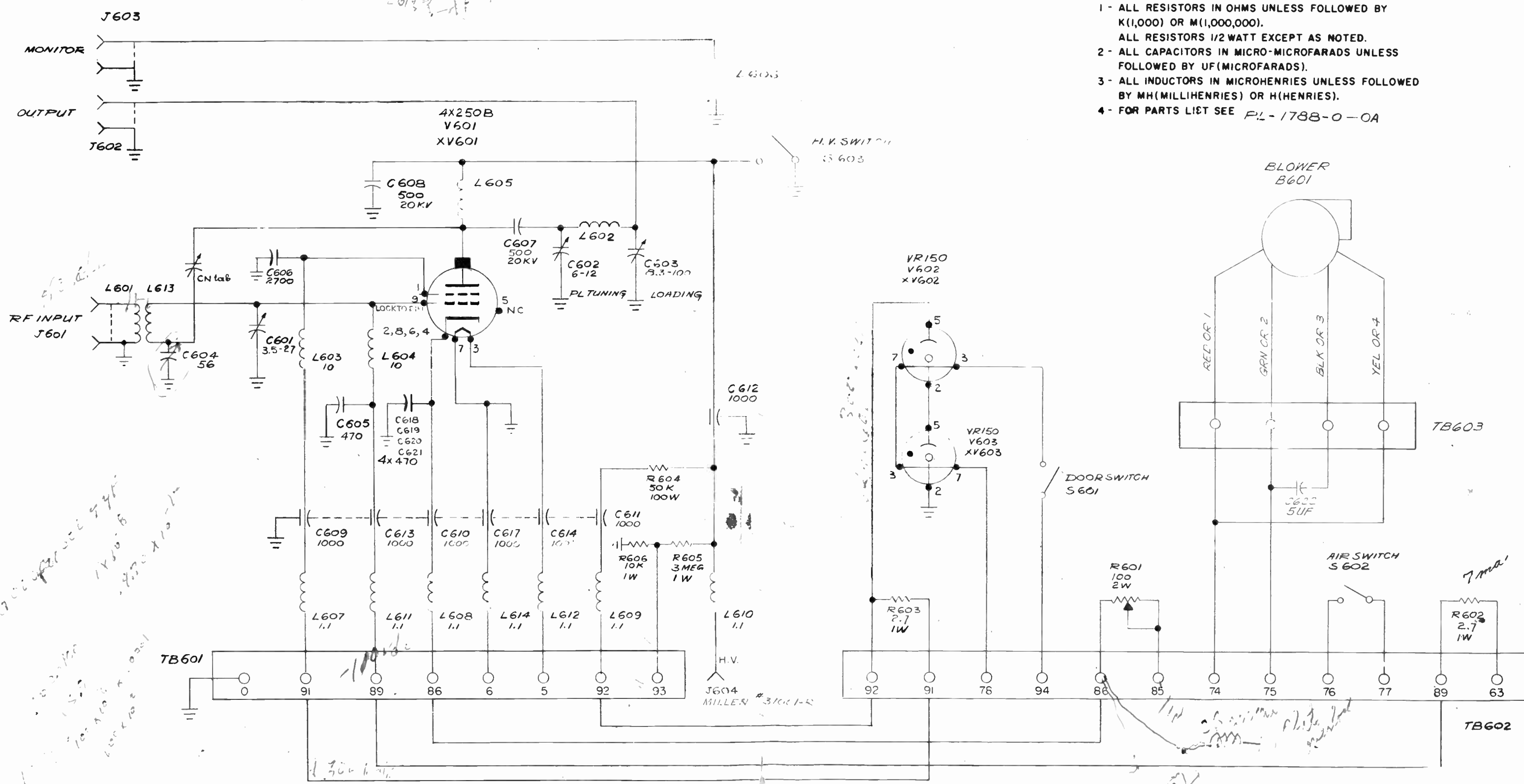
Figure 5-7 S-1788 250W Power Amplifier, schematic diagram
