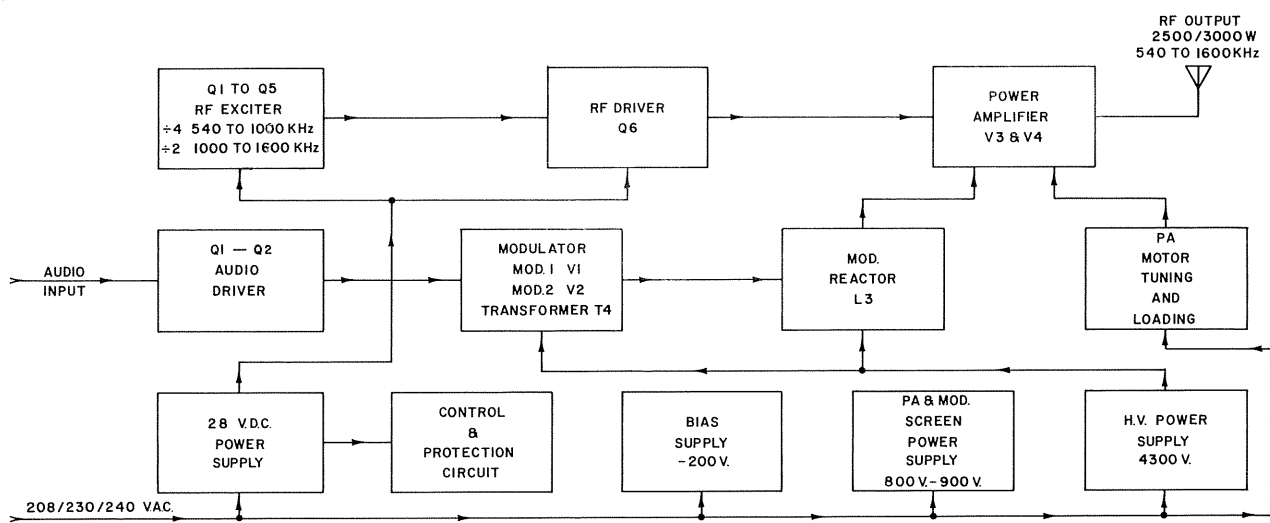
Block diagram
