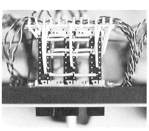
Screw terminal wiring of all inputs—no solder connections
