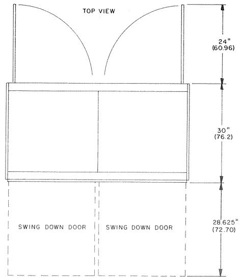
Floor plan
