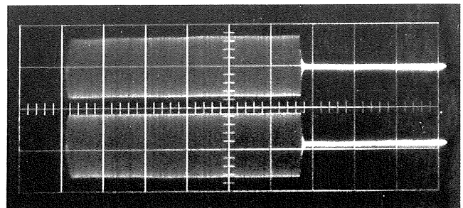
Figure 6: Same input as in Figure 5, but with time base expanded to show the compression ripple more clearly.
