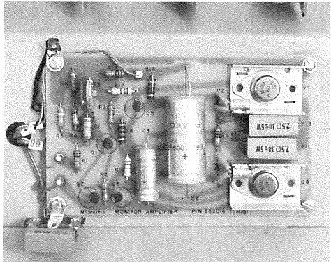
Monitor amplifier
