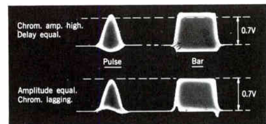
Gain inequality can be measured over the range \pm 3 dB, and delay inequality over the range 110 nsec lag to 110 nsec lead.
