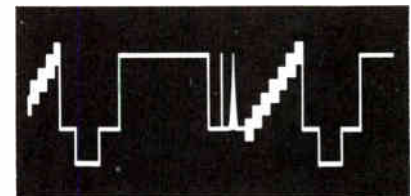
Composite waveform including the chrominance signal super-imposed on the sine-square-pulse and bar.
