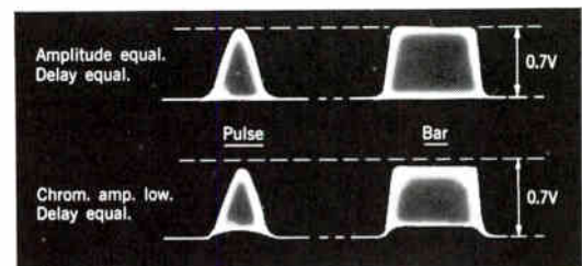
Gain inequality can be measured over the range \pm 3 dB, and delay inequality over the range 110 nsec lag to 110 nsec lead.
