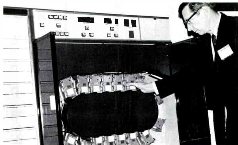
RCA's automated videotape cartridge player.
