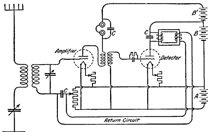
FIG. 62: A Two-Tube Reflex Amplifier. — The order of connecting the instruments in each circuit is very important; and the size of the three by-pass condensers marked C must be carefully chosen. Note how the rectified audio-frequency current from the detector is brought back through the return circuit to the grid circuit of the first tube, to be amplified again before reaching the telephones.
