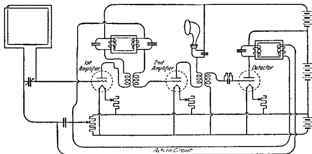
FIG. 63: A Three-Tube Reflex Amplifier. — This is a logical extension of the scheme utilized in Fig. 62; and, with only three tubes, gives detection and four stages of amplification. By-pass condensers of about 0.002 of a microfarad usually work well. Very strong loud-speaker signals cannot be produced without hampering the radio-frequency amplification of the first two tubes.
