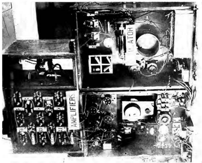
THE RADIO-TELEPHONE TRANSMITTING APPARATUS USED AT ARLINGTON (VA.) FOR THE LONG-DISTANCE EXPERIMENTS OF 1915
