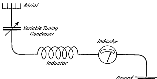
FIG. 43: An Example of Tuning with Variable Condenser. — This is like the receiver of Fig. 41, but has an added variable condenser for tuning. If the inductor is left at a constant value, the resonant frequency of the receiver may be changed by altering the capacitance of the condenser shown. The indicator is, as before, a very sensitive ammeter.
