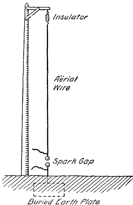
FIG. 5: Marconi's Grounded Transmitter. — The wires from the gap led to a spark coil, as used by Hertz. When sparks jump across the gap, quite powerful radio waves are emitted by the vertical aërial wire.
