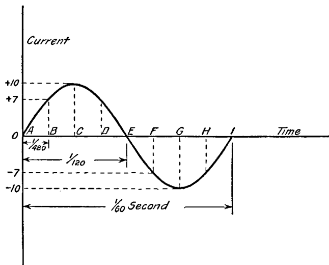
FIG. 20: A Chart of Alternating-Current Flow. — By representing the instantaneous current values (at A, B, C and the following eighth-cycles) of Fig. 19 as vertical lines of appropriate length (7 units upward for instant B, 10 downward for instant G, etc.), we can plot a wavy line showing the current value at any instant. This curve pictures one cycle of a 60-cycle-per-second current; the time of one cycle (from A to I) being \frac{1}{60} of a second, and the time of each eighth-cycle being \frac{1}{480} of a second. Curves of this sort are very useful for showing wave-motions.
