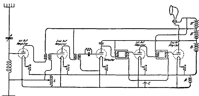
FIG. 61: A Five-Tube Radio-Audio Amplifying Receiver. — This combines the arrangements of Figs 58 and 59. It is a good plan to divide the B battery into three sections, as shown: 20 volts for the detector, 40 for the radio-frequency amplifiers, and 80 for the audio-frequency tubes.
