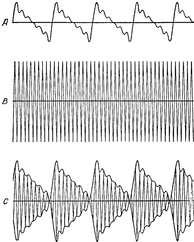
FIG. 30: Combining a Violin Tone and a Radio Wave. — The 2000-cycle violin tone shown at A will mold or modulate the stream of continuous 20,000-cycle radio-frequency current B into the form illustrated at C . The intensity of the radio wave thus produced varies from instant to instant exactly in accordance with the vibrations of the original tone. The principle is the same whether the radio frequency current is of 20,000 cycles, as here drawn, or of 750,000 cycles. Modulation forces it to vibrate between boundaries that are fixed by the tone transmitted.
