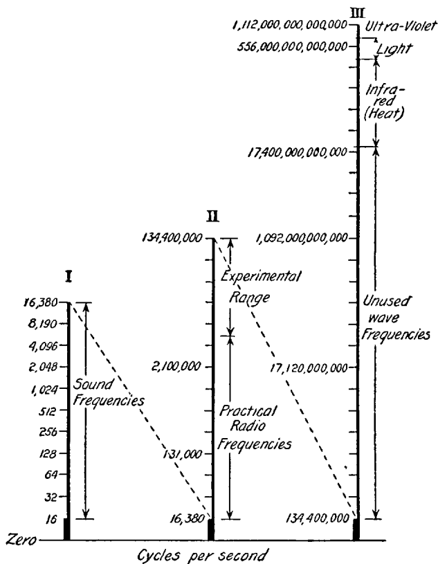
FIG. 16: Radio Frequencies Compared to Light and Sound. — This chart is arranged in octaves, i.e. , each division represents a doubling of frequency. Sounds used in music cover about eight octaves, and audible sounds about ten octaves, as shown by scale I. These are usually air or other mechanical vibrations. Radio frequencies overlap the higher sound frequencies to some extent; but practical values run upward some eight or nine octaves from 16,000 cycles. These are usually electro-magnetic vibrations. Experimental frequencies extend a few octaves higher; and then come about seventeen octaves of frequencies not in everyday use. The whole scale of visible waves (light) extends over only about one octave.
