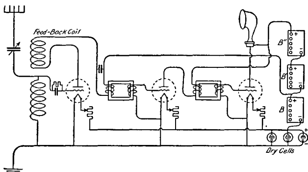
FIG. 65: Regenerator with Two-stage Audio Amplifier. — This is the simple circuit of Fig. 64, combined with the amplifier of Fig. 56, which has been modified by eliminating the 6-volt storage battery A and using 3 WD-11 "dry-cell tubes." Note the three dry cells connected in parallel to supply filament current to all three tubes.
