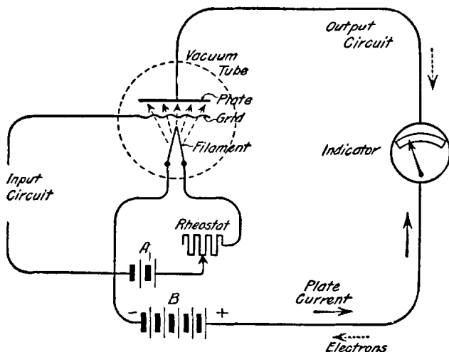
FIG. 50: Fundamental Circuits of the Audion. — The filament is heated by current from the battery marked A; and its temperature controlled by the rheostat shown, as in Fig. 18. The plate-circuit battery B has its positive terminal connected to the plate, and its negative terminal to the filament, thus completing the output circuit containing the indicating device. The current in this output (or plate) circuit is made up of electrons that flow across the space from filament to plate within the vacuum tube, as indicated by the dashed arrows. The direction of electron flow is opposite to that conventionally assumed for electric "current" (positive to negative), as is shown by the solid arrows. By varying the potential applied to the grid by way of the input circuit, the amount of current flowing in the plate circuit (and registered on the indicating meter shown) can be controlled.
