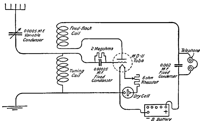
FIG. 64: The Simple Inductively-coupled Regenerator. — This easily built and adjusted circuit is giving excellent results in the hands of thousands of radio novices, and is a good one to begin with.
