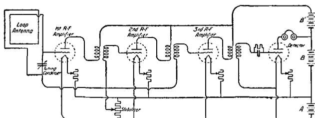
FIG. 60: Three-stage Radio-Frequency Amplifier, with Audion Detector. — The loop antenna and its tuning condenser are equivalent in many ways to the secondary circuit shown in earlier figures. Here the feeble radio currents generated in the loop are amplified three times before reaching the detector. Common batteries and stabilizer are used, as in Fig. 59.
