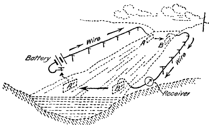
FIG. 1: How Morse Telegraphed across a Canal. — When the key was pressed, current from the battery flowed along the wire on the left-hand bank, across the canal through the water from submerged plate A to B (in the distance), back along the wire on the right-hand bank, through the receiver, and across the canal again from plate B' to A' . Some current was lost by diffusing from A to A' , but enough reached the receiver to operate it.
