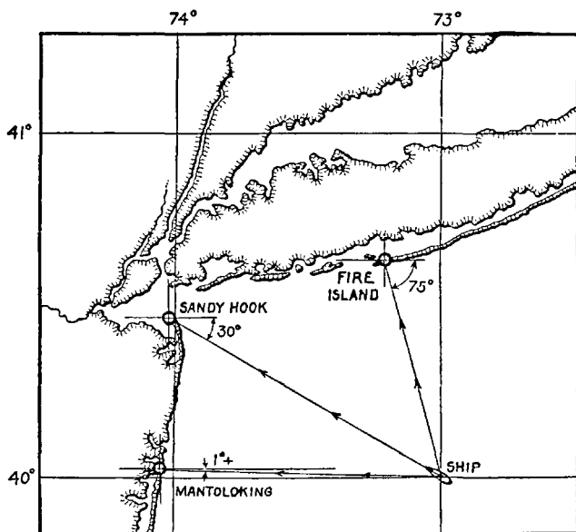
FIG. 66: Determining a Ship's Position by Radio. — The Radio Compass station at Fire Island finds that radio signals from the ship illustrated, come in along a line 75^\circ south of east. Sandy Hook hears the same signals along the line running 30^\circ south of east. When these two lines are drawn on a chart, their point of crossing will be found to be at 73^\circ longitude and 40^\circ latitude, which is the ship's position while sending. A third observation from Mantoloking (in this case a little over 1^\circ south of east) will check the other two readings. If the three lines cross in a single point, the determination is accurate; but if they enclose a large triangle, the position of the ship will not be definitely known.
