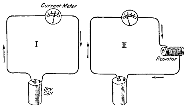
FIG. 17: The Effect of Resistance. — The simple circuit at I passes 3 amperes as shown by the meter. When a resistor of \frac{1}{2} an ohm is inserted in the circuit, as at II, the 1½ volt dry cell can force only 1½ amperes through the circuit. The arrows indicate the direction of current flow, according to the usual convention.
