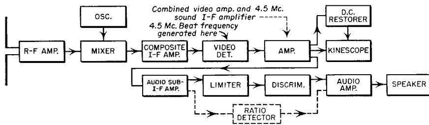
INTER-CARRIER SOUND TV RECEIVER FIG. 3
