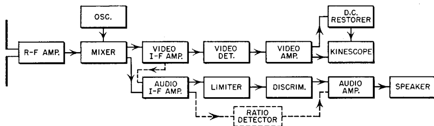
CONVENTIONAL DUAL-I-F TV RECEIVER FIG. 2
