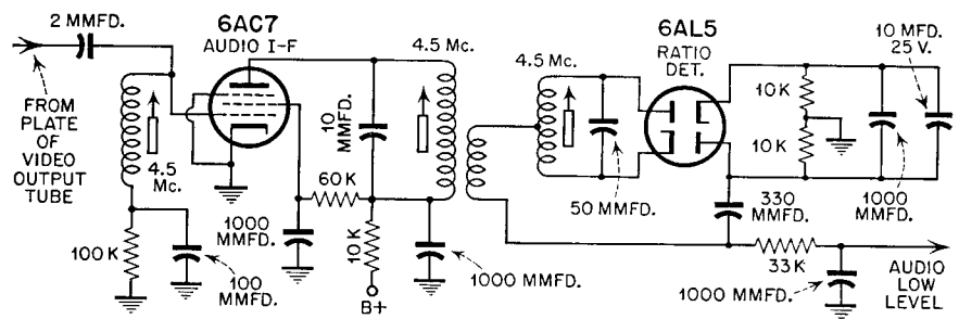
4.5 Mc. CIRCUITS FOR INTER-CARRIER SOUND FIG. 6
