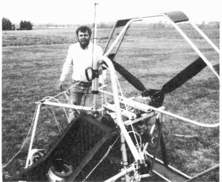
Close-up view of the PVC antenna mount attached to the ultralight. John N3JRE in the background.
