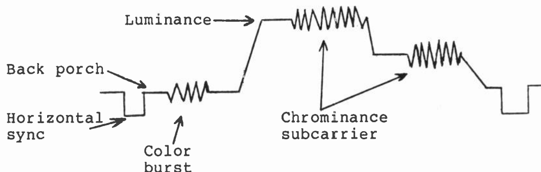
Fig. 1. Composit video signal.
