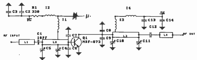
Figure 2 Schematic diagram of MRF-873. Microstriplines are reproduced from board print
