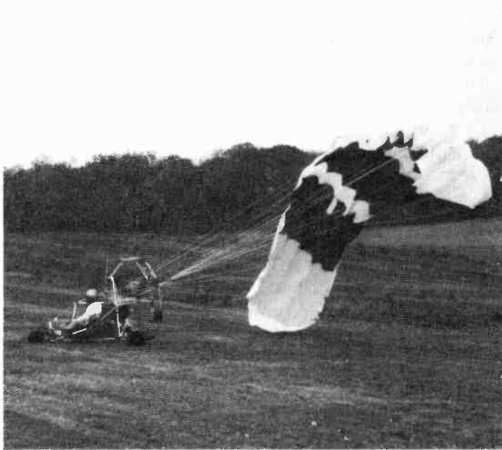
Takeoff of the Ultralight ATV mobile station with John N3JRE at the controls. The paraglider only takes a few hundred feet to takeoff.
